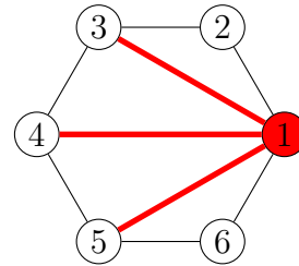
(b) Triangulation with vertex 1 as root
