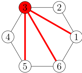
(a) Triangulation with vertex 3 as root
