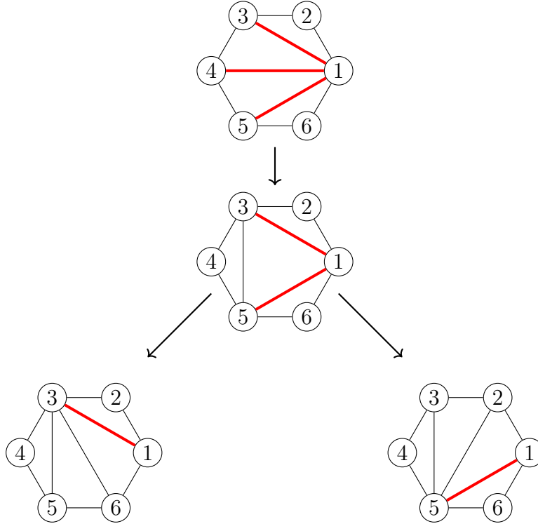
Figure 7: Four hexagons showing transformation paths in the genealogical tree. Top: Root triangulation with chords (1, 3) , (1, 4) , (1, 5) . Middle: After flipping (1, 4) , we obtain chord (3, 5) . Bottom-left: From middle, flipping (1, 5) yields (3, 6) . Bottom-right: From middle, flipping (1, 3) yields (2, 5) . Each transformation involves flipping exactly one generating chord (red), demonstrating the parent-child relationships in the local genealogical tree.
