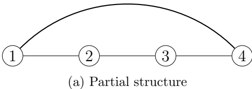
Figure 10: (a) and (b) show two separate structures formed by vertices \{v_{i+1}, \dots, v_{j-1}\} and \{v_{j+1}, \dots, v_{i-1}\} , respectively. Each structure is a simple path, ensuring that at least one endpoint in each structure can serve as a safe root vertex.
