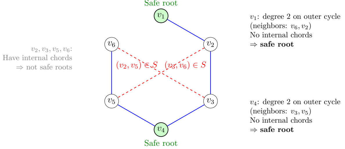
Figure 1: Illustration of Theorem 1: A hexagonal face with two existing chords (v_2, v_5) and (v_3, v_6) from previously processed faces (red dashed lines). Viewing this as an outerplane graph, vertices v_1 and v_4 have degree 2 on the outer cycle (blue boundary) with no incident internal edges. By the classical theorem, at least two such vertices exist, guaranteeing safe roots for algorithm initialization.
