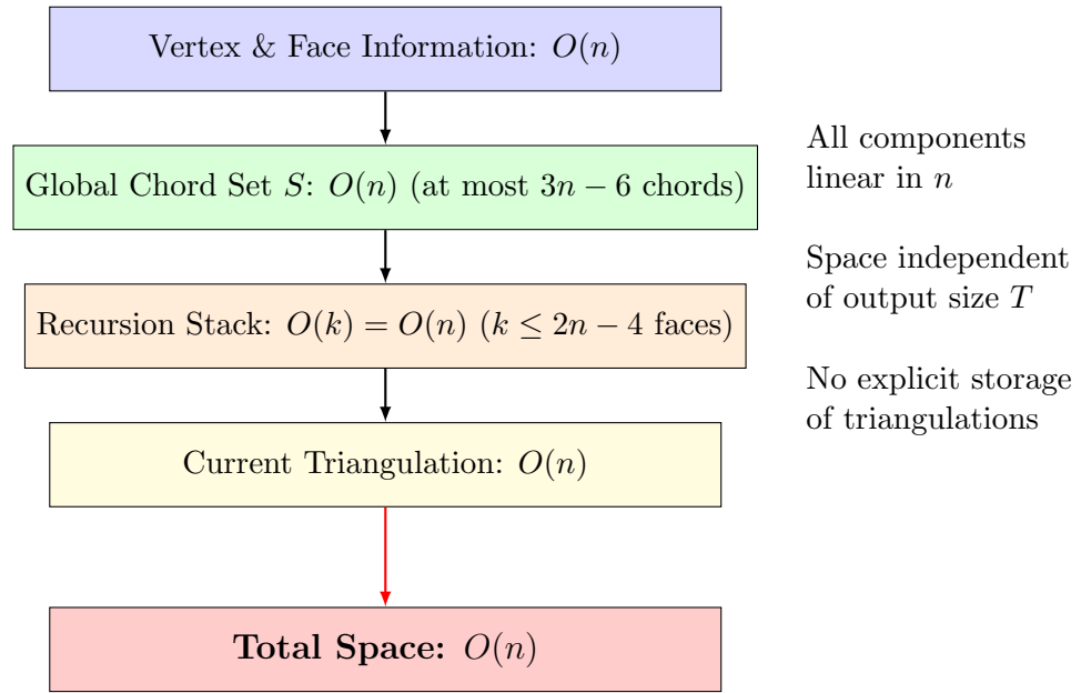
Figure 14: Space complexity breakdown. All data structures use O(n) space: vertex/face information, global chord set S (bounded by planarity), recursion stack (bounded by Euler's formula), and current triangulation storage. Critically, space usage is independent of the number of triangulations T , which can be exponential in n . The algorithm generates triangulations on-the-fly without storing all of them.
