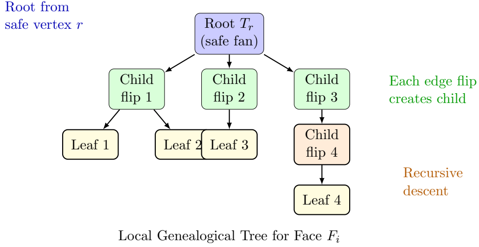
Figure 6: Structure of a local genealogical tree for a single face. The root is constructed from a safe root vertex using a fan triangulation. Each child is obtained by flipping the generating chord (leftmost non-root chord). The tree structure ensures each triangulation appears exactly once, with unique parent-child relationships defined by edge flips.
