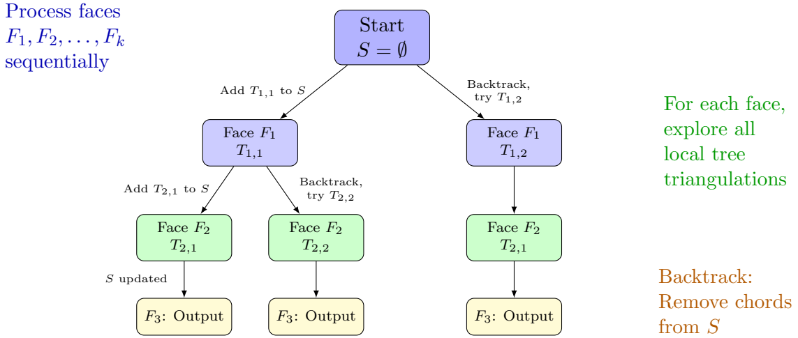
Figure 5: DFS recursion structure with backtracking. The algorithm processes faces sequentially, exploring all triangulations in each face’s local genealogical tree. The global chord set S is updated when entering a branch (add chords) and restored when backtracking (remove chords). Each path from root to leaf represents a unique complete triangulation of the graph.
