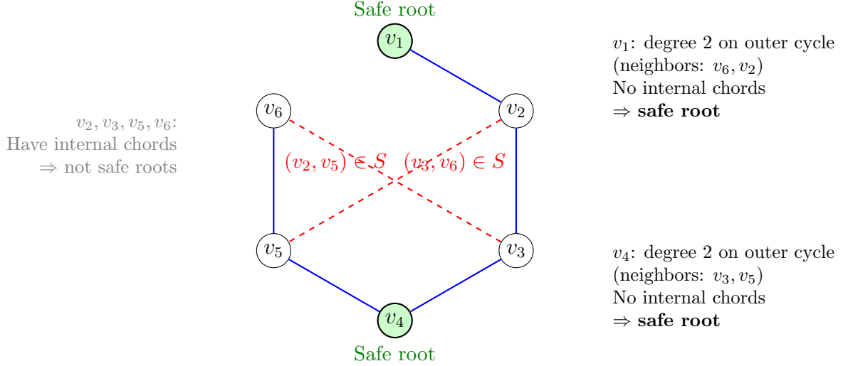
Figure 11: Illustration of Theorem 1: A hexagonal face with two existing chords (v_2, v_5) and (v_3, v_6) from previously processed faces (red dashed lines). Viewing this as an outerplane graph, vertices v_1 and v_4 have degree 2 on the outer cycle (blue boundary) with no incident internal edges. By the classical theorem, at least two such vertices exist, guaranteeing safe roots for algorithm initialization.
