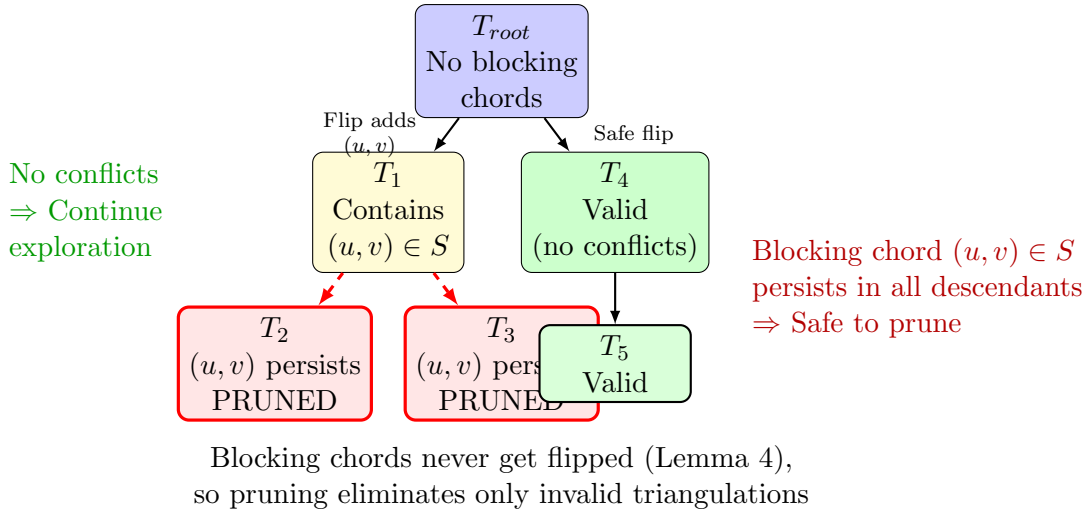
Figure 12: Illustration of Lemma 4: Blocking chord persistence. When a triangulation T_1 contains a chord (u, v) that already exists in the global set S (a blocking chord), this chord cannot be the generating chord and thus persists in all descendants T_2, T_3, \dots . Creating multi-edges in all descendants. Therefore, pruning this entire subtree (red dashed edges) is safe and eliminates only invalid triangulations.
