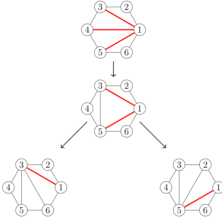
Figure 8: Four hexagons showing transformation paths in the genealogical tree. Top: Root triangulation with chords (1,3) , (1,4) , (1,5) . Middle: After flipping (1,4) , we obtain chord (3,5) . Bottom-left: From middle, flipping (1,5) yields (3,6) . Bottom-right: From middle, flipping (1,3) yields (2,5) . Each transformation involves flipping exactly one generating chord (red), demonstrating the parent-child relationships in the local genealogical tree.
