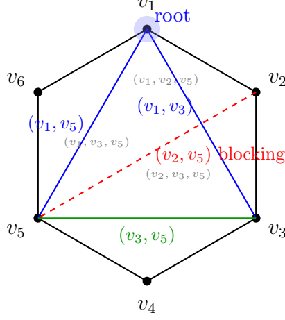
Figure 4: Illustration of Lemma 2: A hexagonal face with triangulation T containing blocking chord (v_2, v_5) (red dashed). The root is v_1 (blue circle). Chords from the root are shown in blue, and other chords in green. The blocking chord forms triangles with vertices v_p = v_1 (root) and v_q = v_3 , preventing it from being the generating chord by Case 3 of the proof.
