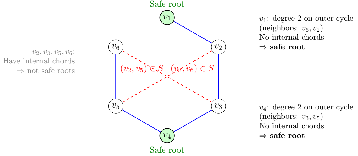
Figure 3: Illustration of Theorem 1: A hexagonal face with two existing chords (v_2, v_5) and (v_3, v_6) from previously processed faces (shown in red dashed lines). Viewing this as an outerplanar graph, vertices v_1 and v_4 have degree 2 on the outer cycle (blue boundary) with no incident internal edges. By the classical theorem, at least two such vertices exist, guaranteeing safe roots for algorithm initialization.
