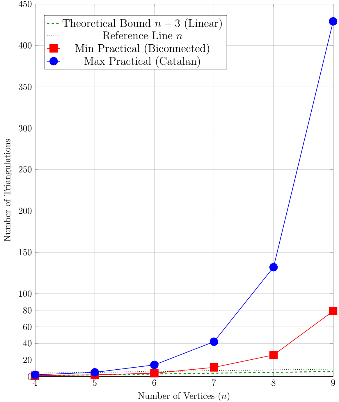
Figure 6: Comparison of theoretical and practical triangulation bounds for n = 4 to n = 9 . Key insight: The minimum practical triangulations (red squares) always exceed the theoretical lower bound n - 3 (green dashed line), confirming that our O(n) lower bound holds even in the worst case. The gap between theory and practice grows exponentially, showing the algorithm performs much better than the theoretical minimum.
