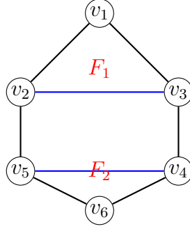
Figure 2: Modified diamond graph with F_1 = \langle v_1, v_2, v_3 \rangle (triangle) and F_2 = \langle v_2, v_3, v_4, v_5 \rangle (quadrilateral).
