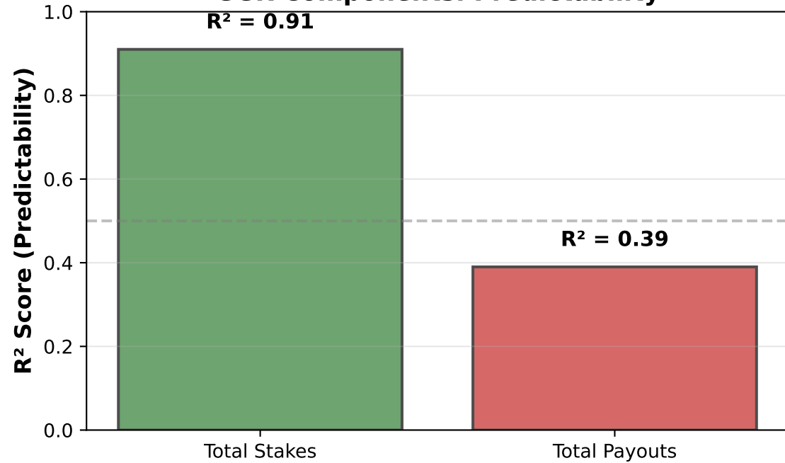
GGR Components: Predictability
