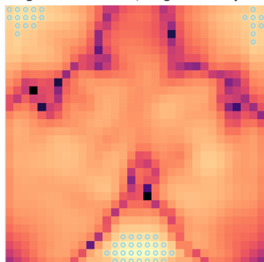
exact influence |dj/dp| , log scale bright = influential; rings: true top 50
