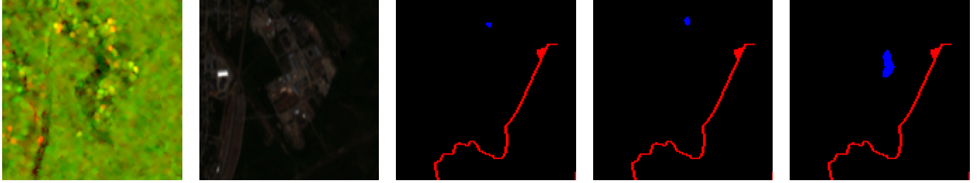
(a) Input Image: SAR (b) Input Image: Optical (c) FN/FP Map: Fusion (d) FN/FP Map: Optical (e) FN/FP Map: SAR Fig. 4: EMSR441_AOI05_2_3_2_2: Fusion(IoU 0.0), Optical(IoU 0.0), SAR(IoU 0.0). A low-coverage tile with a thin riverine flood. All three models miss the channel and share a false-positive region in the upper centre. Fusion inherits the limitation of both baselines.
