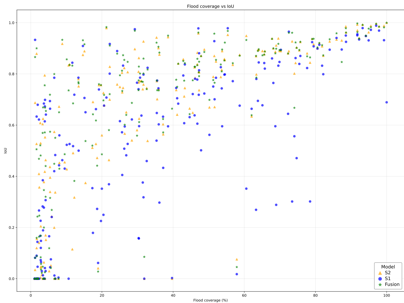
Fig. 16: IoU versus flood coverage for all three models, showing that per-sample IoU rises with the proportion of the tile flooded and collapses on low-coverage tiles.
