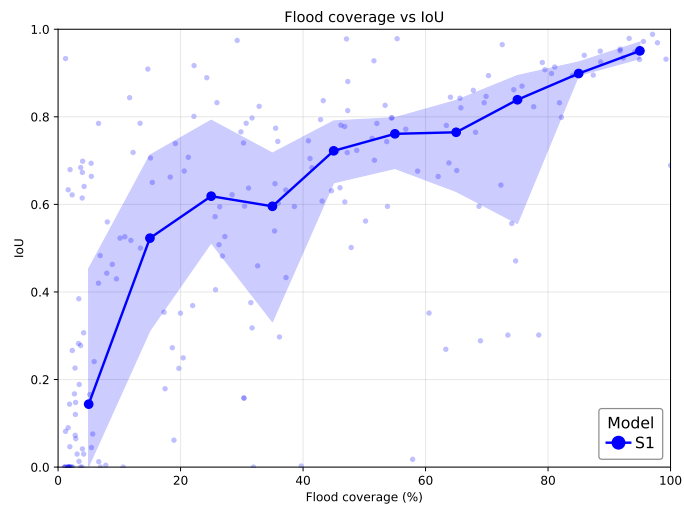
(c) Sentinel-1 (SAR).
