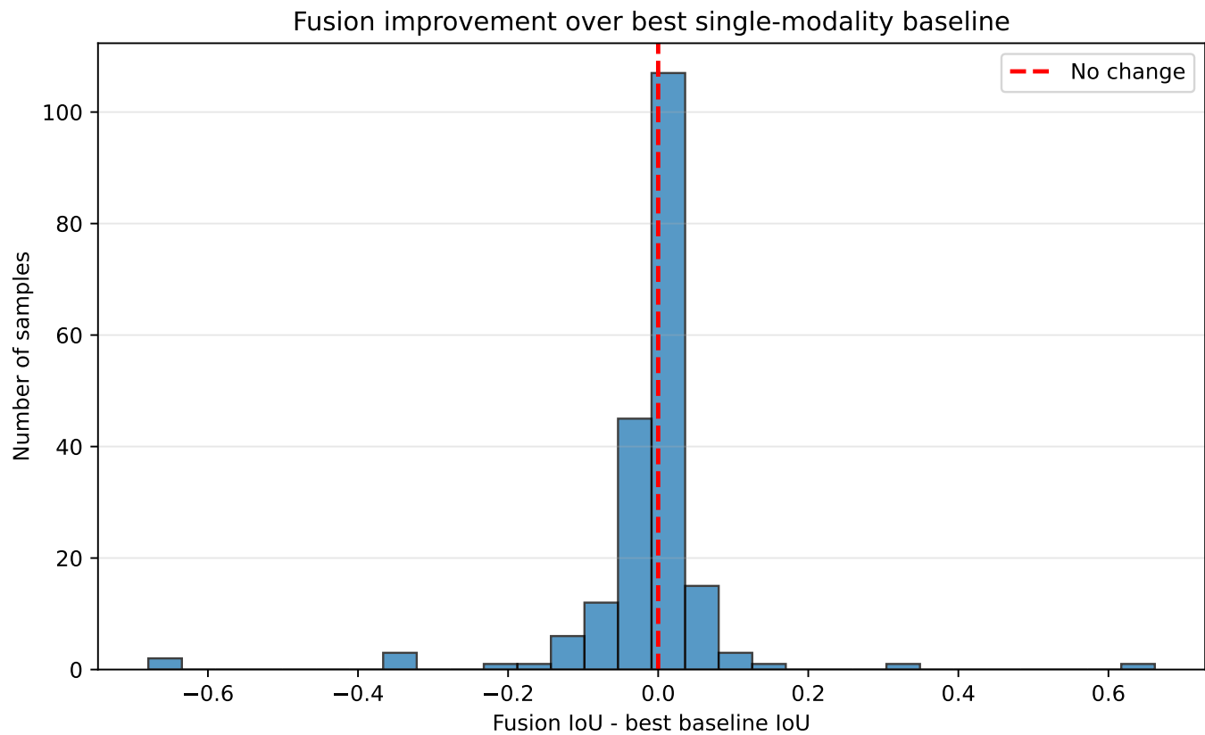
Fig. 24: Distribution of per-sample IoU improvement of the fusion model over the best single-modality baseline.
