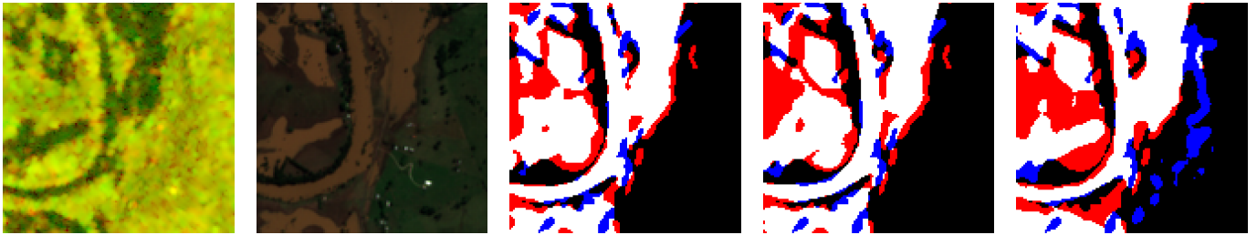
(a) Input Image: SAR (b) Input Image: Optical (c) FN/FP Map: Fusion (d) FN/FP Map: Optical (e) FN/FP Map: SAR Fig. 5: EMSR570_AOI02_07_03_2_1: Fusion(IoU 0.6983), Optical(IoU 0.6693), SAR(IoU 0.5619). A balanced tile with an irregular, visually complex flood boundary. Gives a clear ordering of the three models; fusion outperforms both baselines.
