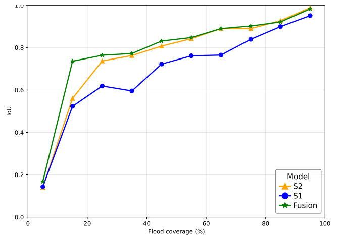
Fig. 2: Median per-sample IoU versus flood coverage for all three models, computed in 10% coverage bins.
