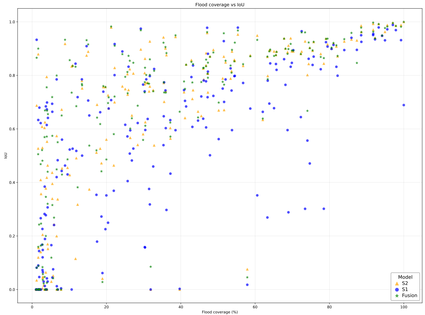
Fig. 18: IoU versus flood coverage for all three models, showing that per-sample IoU rises with the proportion of the tile flooded and collapses on low-coverage tiles.
