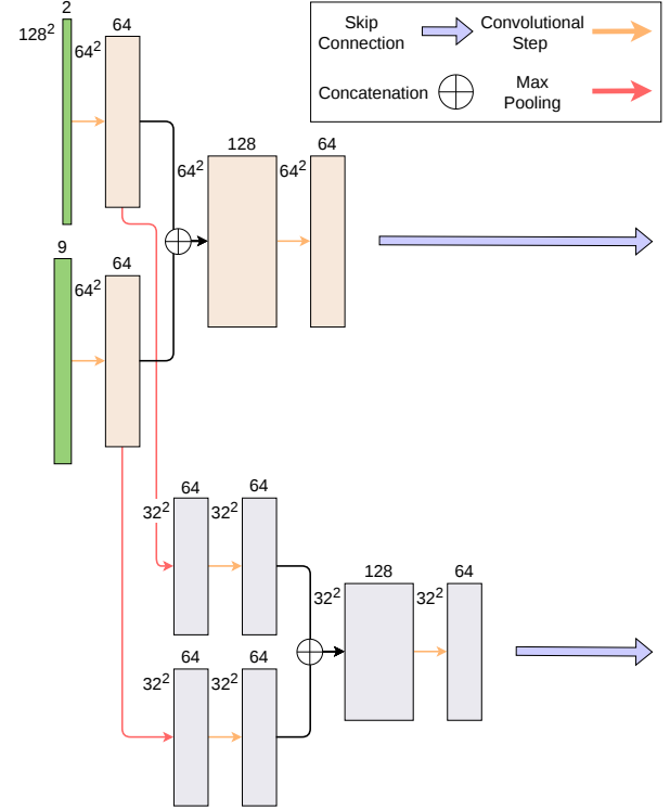
Fig. 1: Feature-fusion parallel-encoder design, showing the first two of the network’s encoder levels. The S1 (SAR, VV/VH) and S2 (optical, 9-band) inputs are processed by separate ResNet-34 encoder streams and fused at each level by concatenation followed by a 1 \times 1 convolution.
