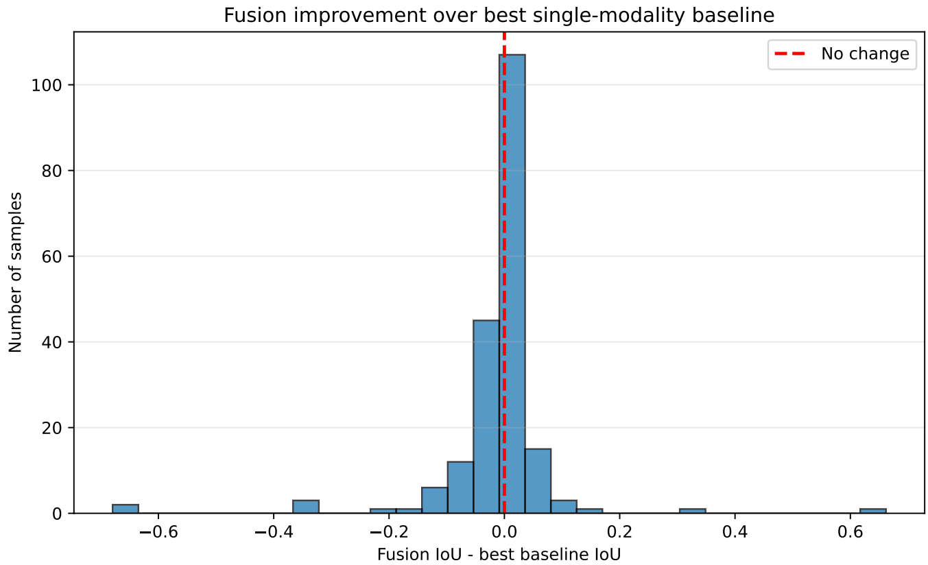
Fig. 26: Distribution of per-sample IoU improvement of the fusion model over the best single-modality baseline.
