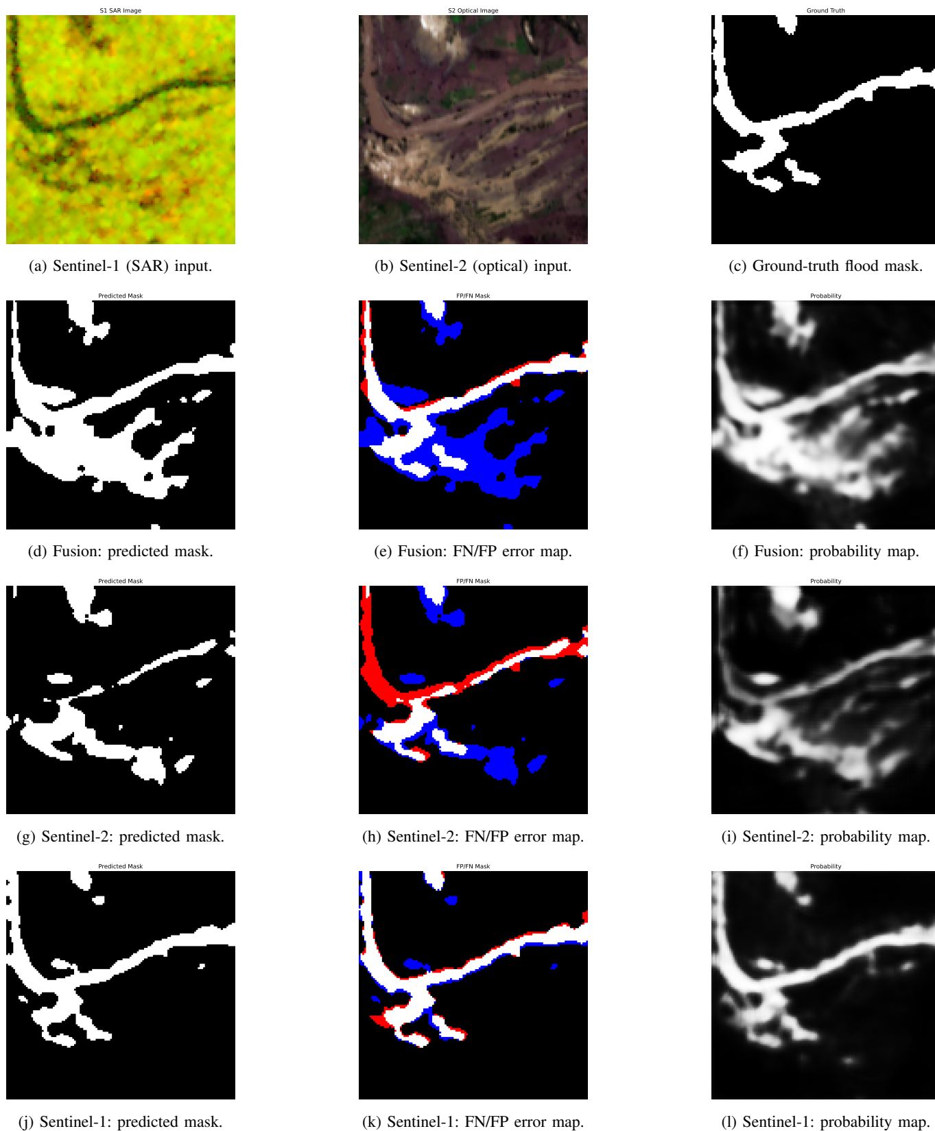
Fig. 24: EMSR470_AOI01_47_10_1_2: Fusion (IoU 0.3818), Optical (IoU 0.3173), SAR (IoU 0.7187). SAR substantially outperforms both other models, cleanly capturing the narrow channel. Fusion improves slightly on optical, showing some SAR benefit, but the strong optical signal limits the gain and fusion falls well short of SAR.
