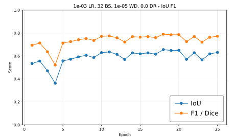
(c) IoU and F1 score.
