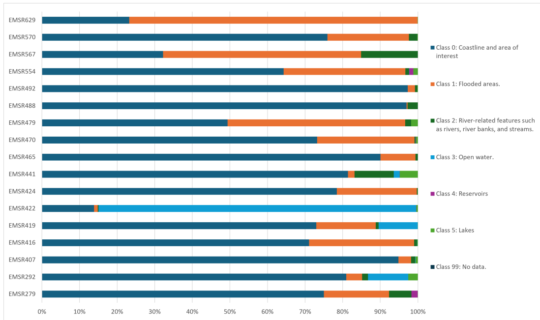
Fig. 8: Per-event class composition from the original STURM-Flood multi-class labels, shown before conversion to the binary water/non-water masks used in this work. Class balance varies considerably across events.
