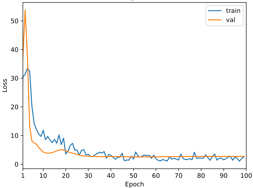
Training Curves
