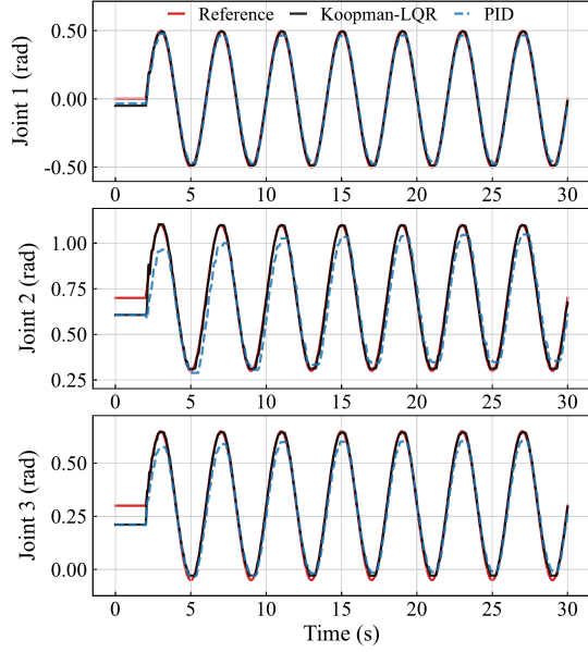
Fig. 5. Comparison of the sinusoidal trajectory tracking performance of the Koopman-LQR and the PID Controllers.
