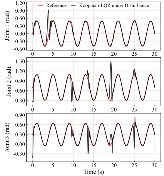
Fig. 7. Robustness test under disturbances.
