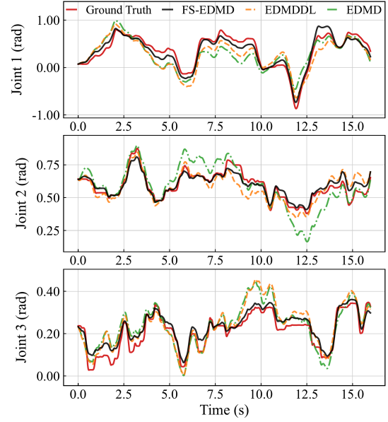
Fig. 4. Comparison of the joint position prediction results obtained by FS-EDMD, EDMDDL, and the standard EDMD.
