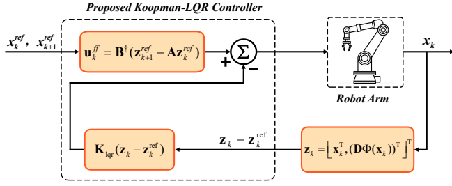
Fig. 2. The proposed Koopman-based feedforward-feedback LQR control structure.
