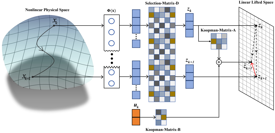
Fig. 1. Koopman representation learning with the learnable feature selection mechanism.
