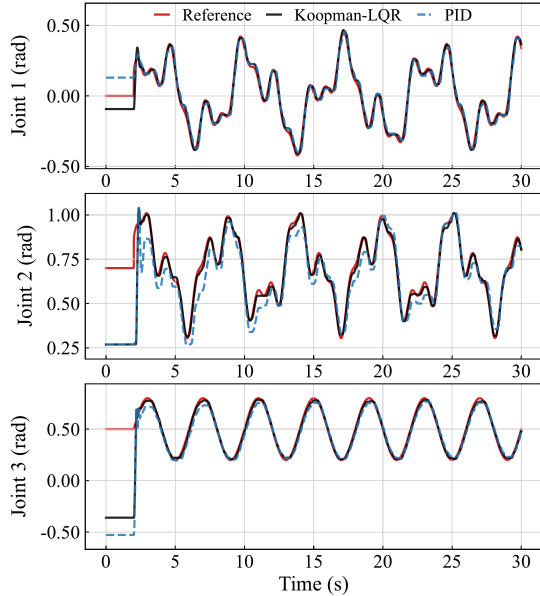
Fig. 6. Comparison of the irregular trajectory tracking performance of the Koopman-LQR and the PID Controllers.
