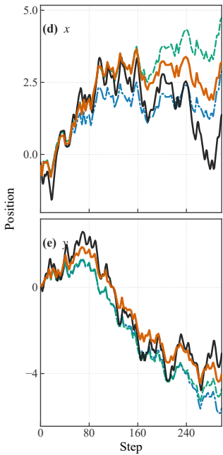
— Ground truth — FS-EDMD - - EDMDDL - - EDMD Robotic arm Soft platform
