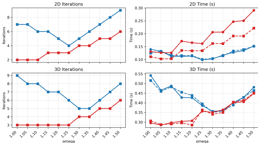
CUDA MG omega sweep - sine 2D grid=4095, 3D grid=383
