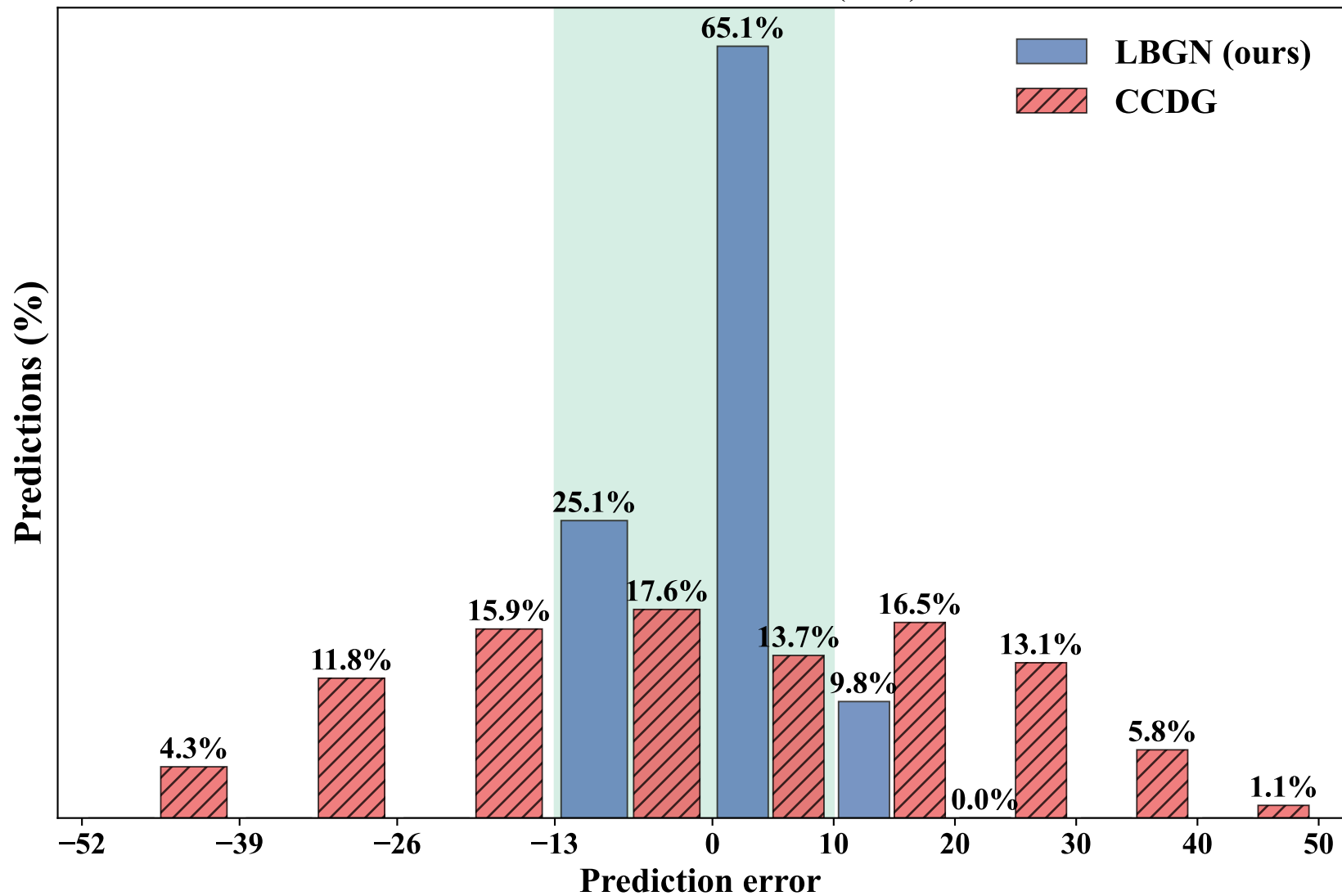
N-CMAPSS: D4→D1 (best)
