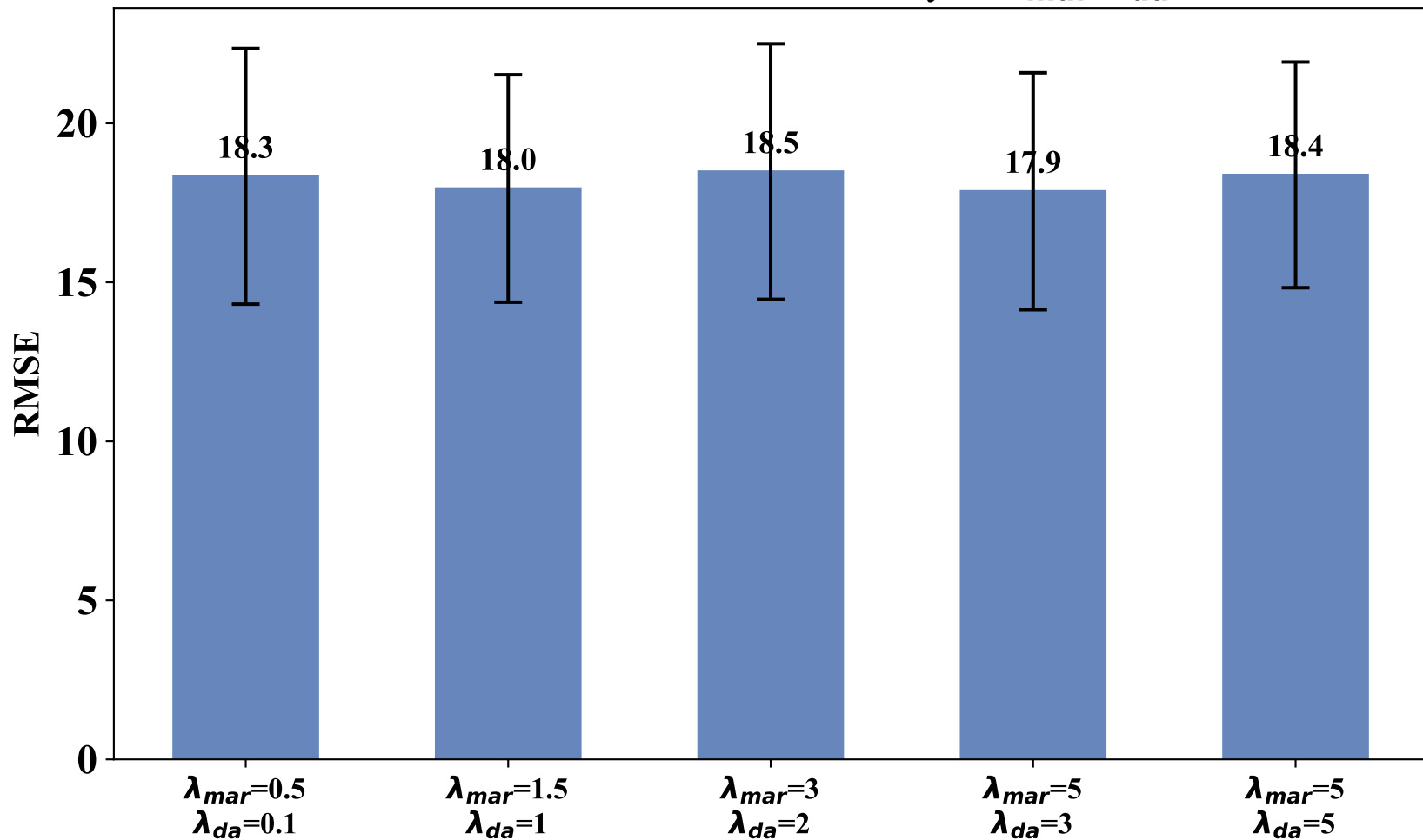
CMAPSS: LBGN-RUL sensitivity to \lambda_{mar}/\lambda_{da}
