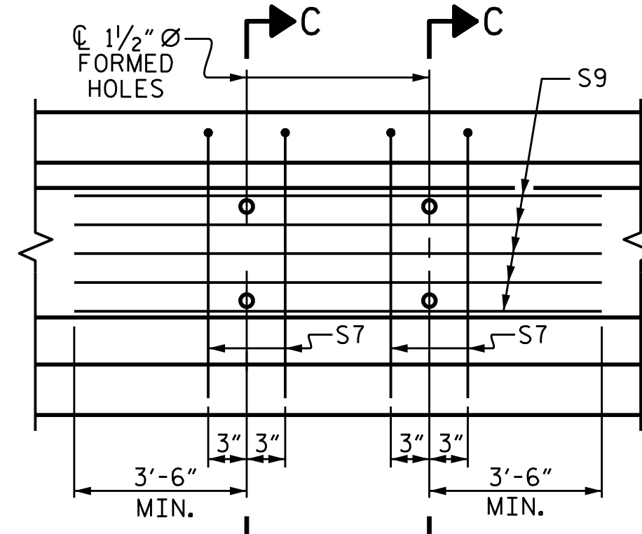
PARTIAL ELEVATION
