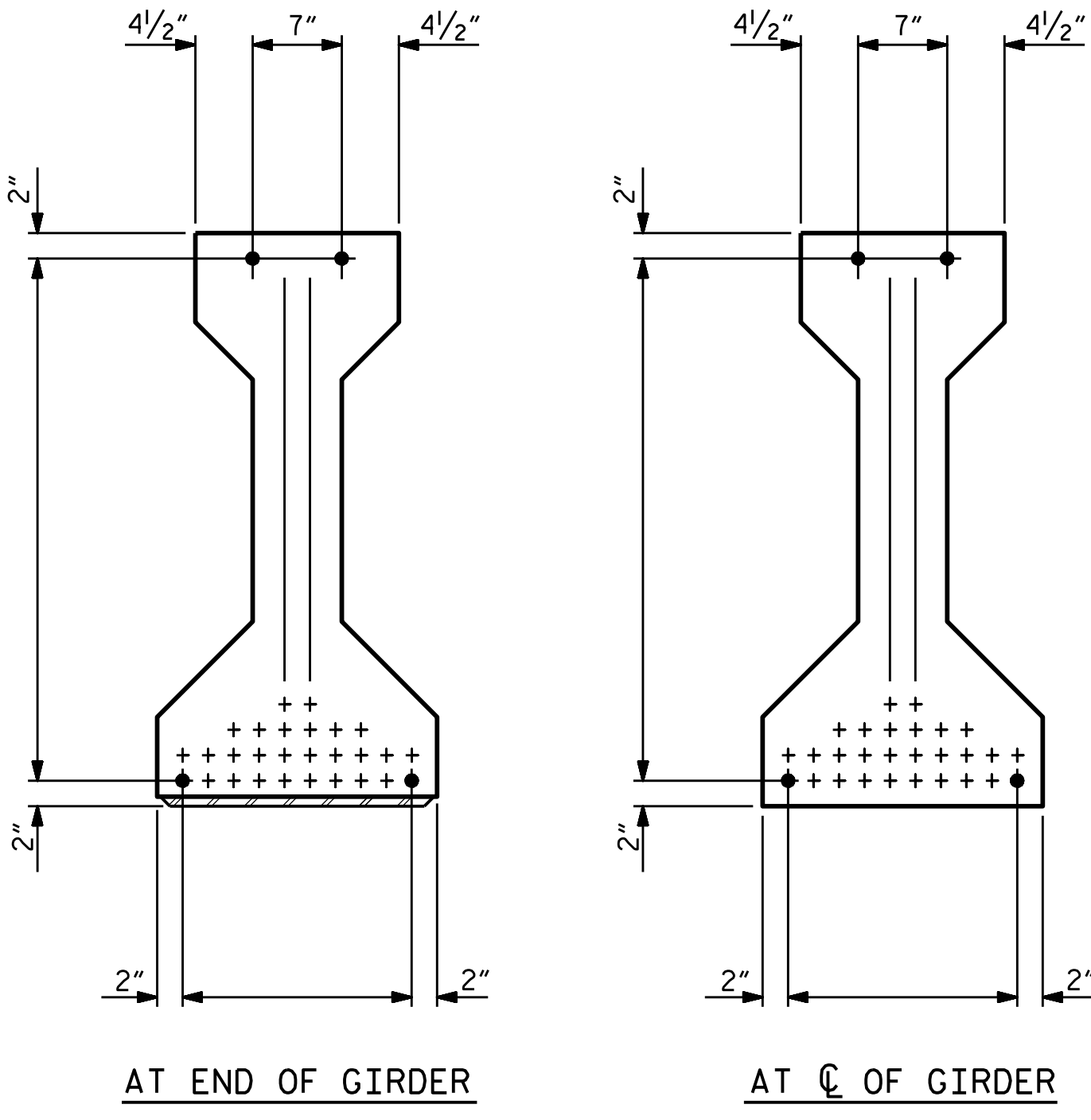
0.6" Ø LOW RELAXATION STRAND LAYOUT
