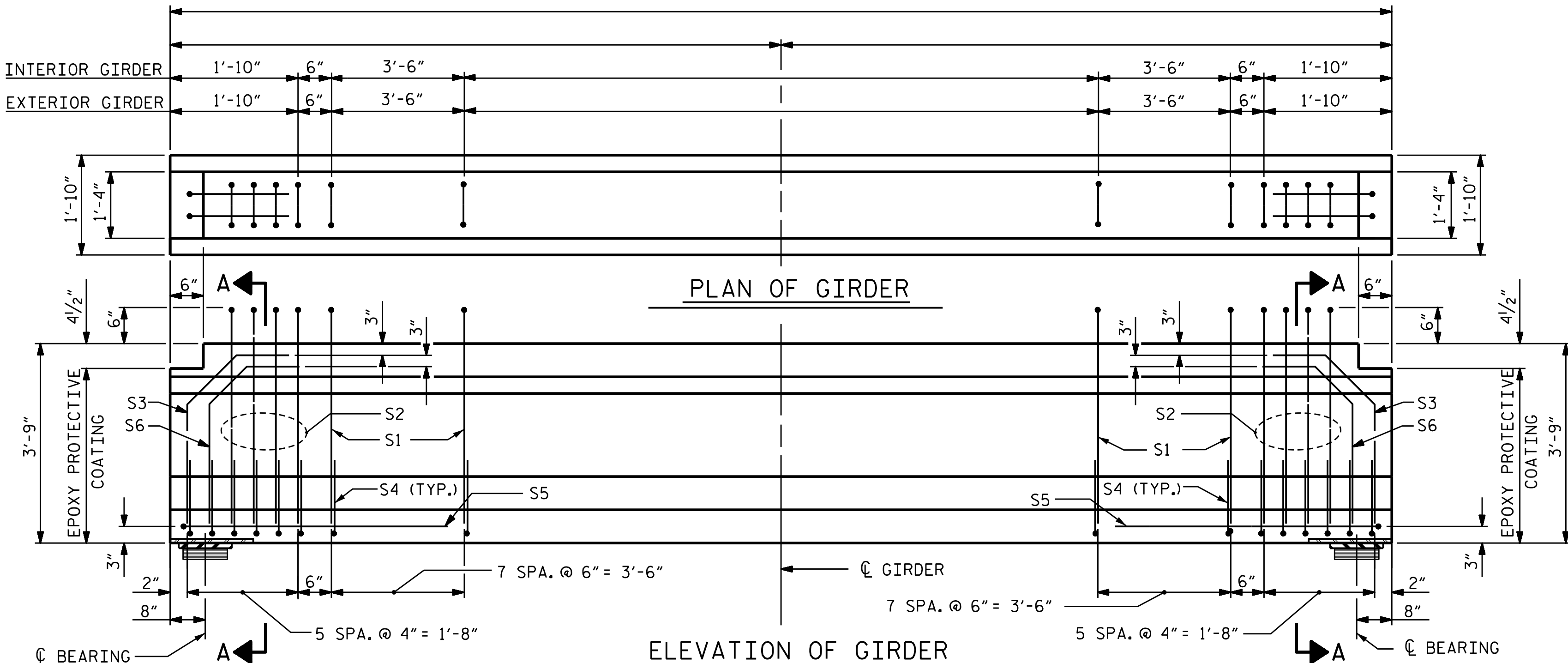
(SEE PARTIAL ELEVATION FOR ADDITIONAL "S" BARS)
