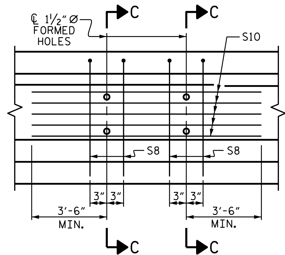
PARTIAL ELEVATION SHOWING INTERMEDIATE DIAPHRAGM REINFORCING STEEL FOR GIRDER Nos. ----- (FOR INTERIOR GDRS. WITH SKEW < 70° OR SKEW > 110°)
