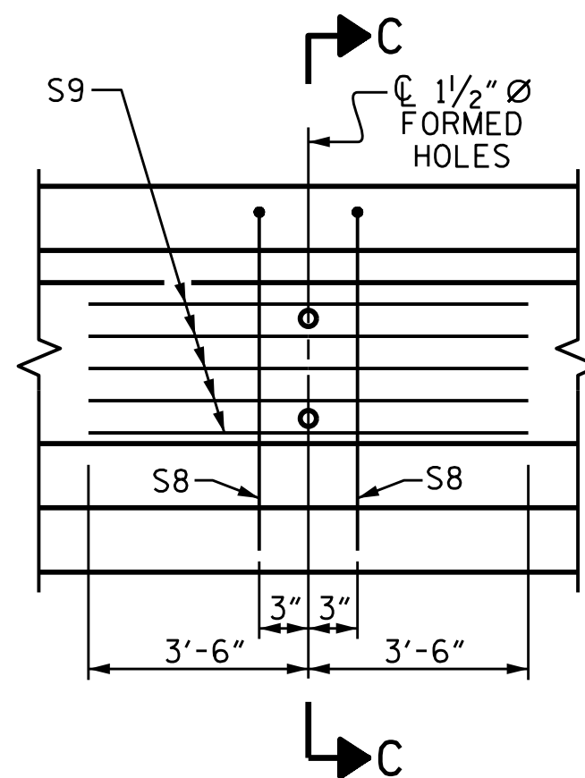
PARTIAL ELEVATION SHOWING INTERMEDIATE DIAPHRAGM REINFORCING STEEL FOR GIRDER Nos. ----- (FOR ALL EXTERIOR GIRDERS AND INTERIOR GIRDERS WITH 70° ≤ SKEW ≤ 110°)
