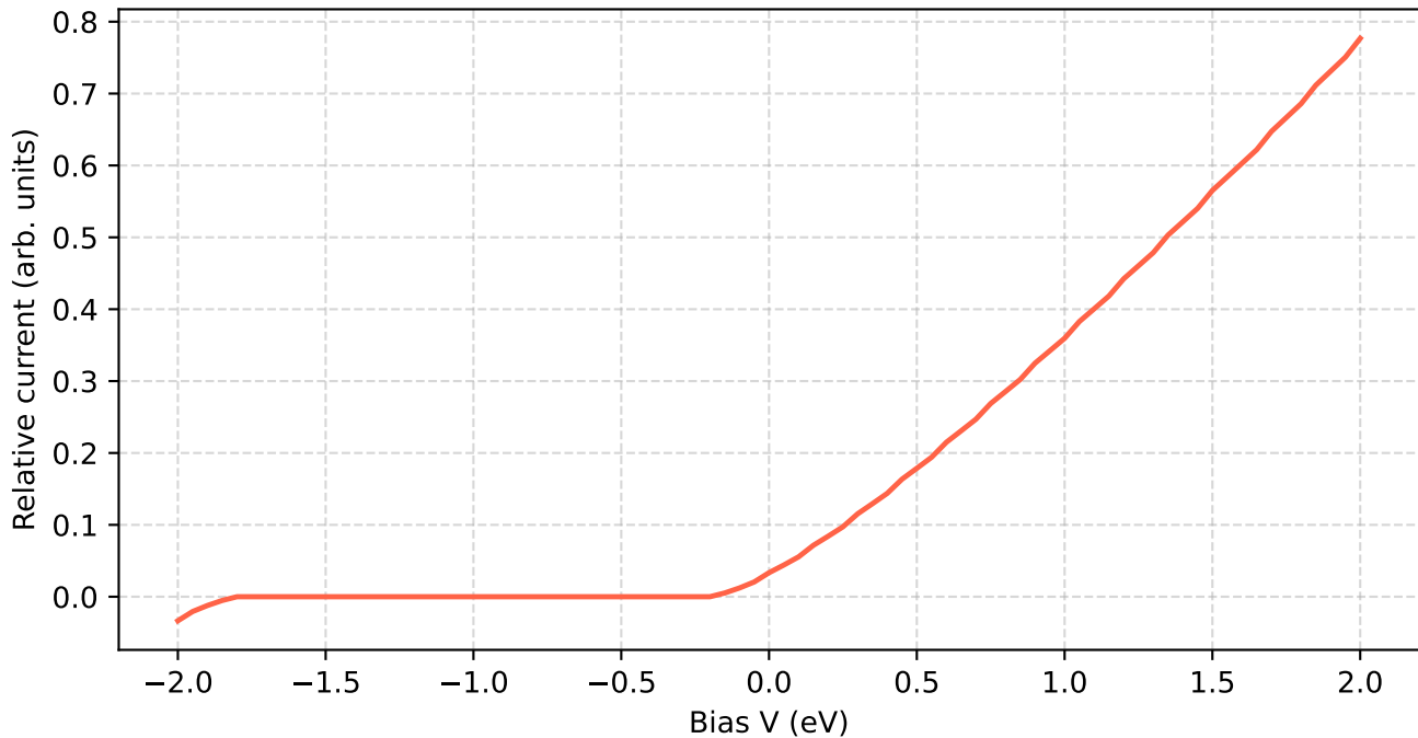
I-V of CNT heterojunction (Schottky-like rectification)
