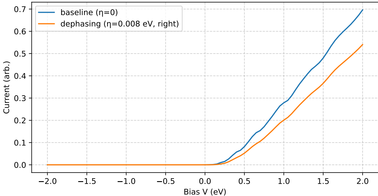
I-V of CNT-like Schottky diode @300K
