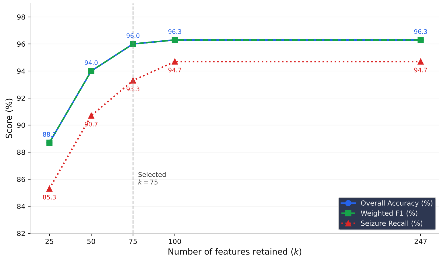
Feature-Count Ablation — RF60+SVM40\_C2 (Validation Set)
