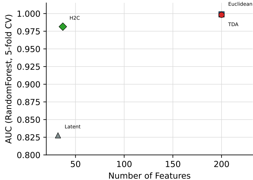
(B) Features vs Performance
