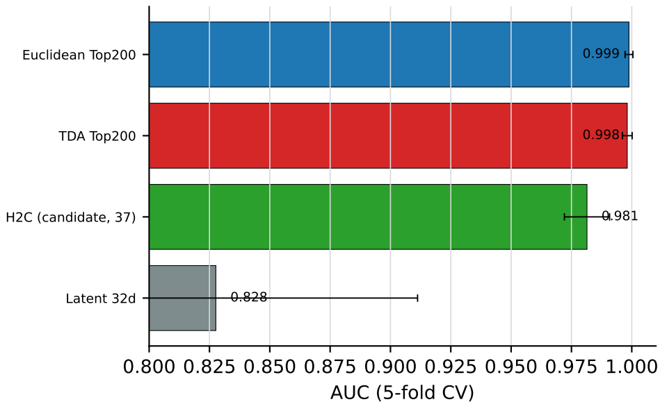
(A) Classification: AUC (RandomForest, fold-internal CV)
