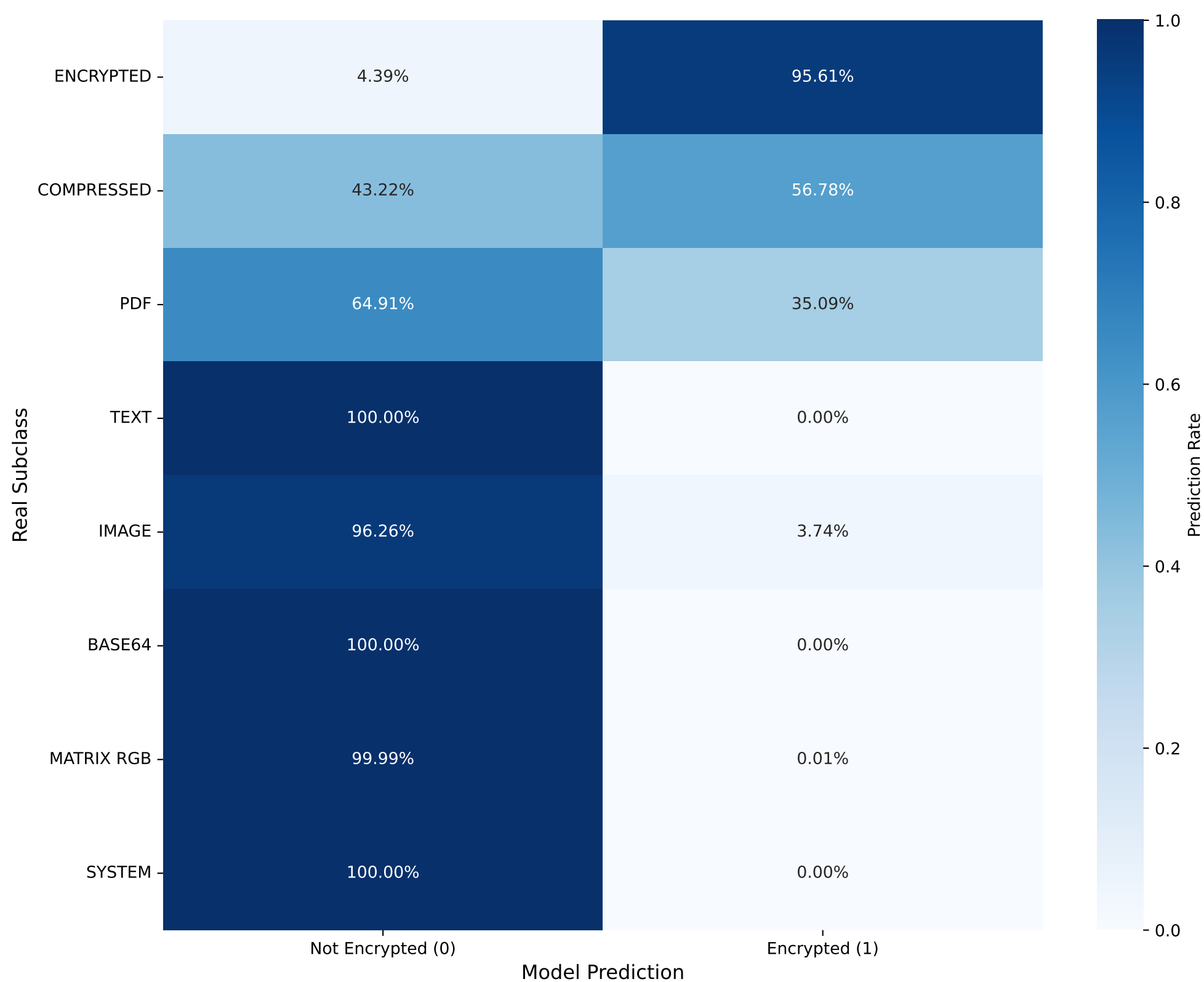
Confusion Matrix by Subclasses
