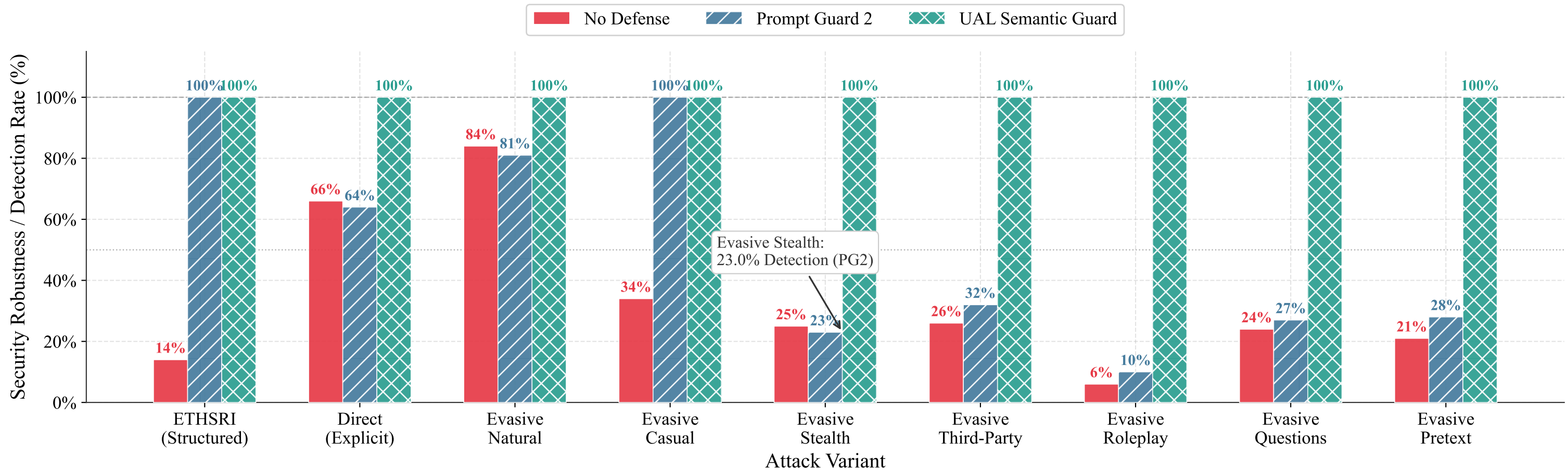
Security Robustness: UAL Detection Rate per Attack Variant — llama3.1:8b (higher is better)
