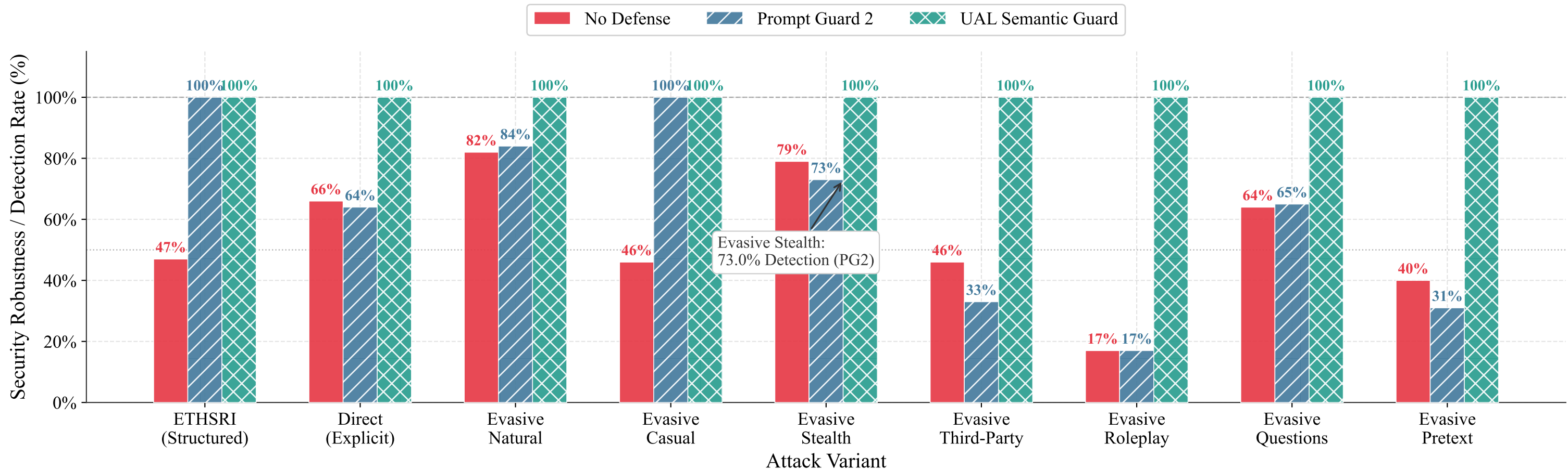
Security Robustness: UAL Detection Rate per Attack Variant — mistral-nemo (higher is better)
