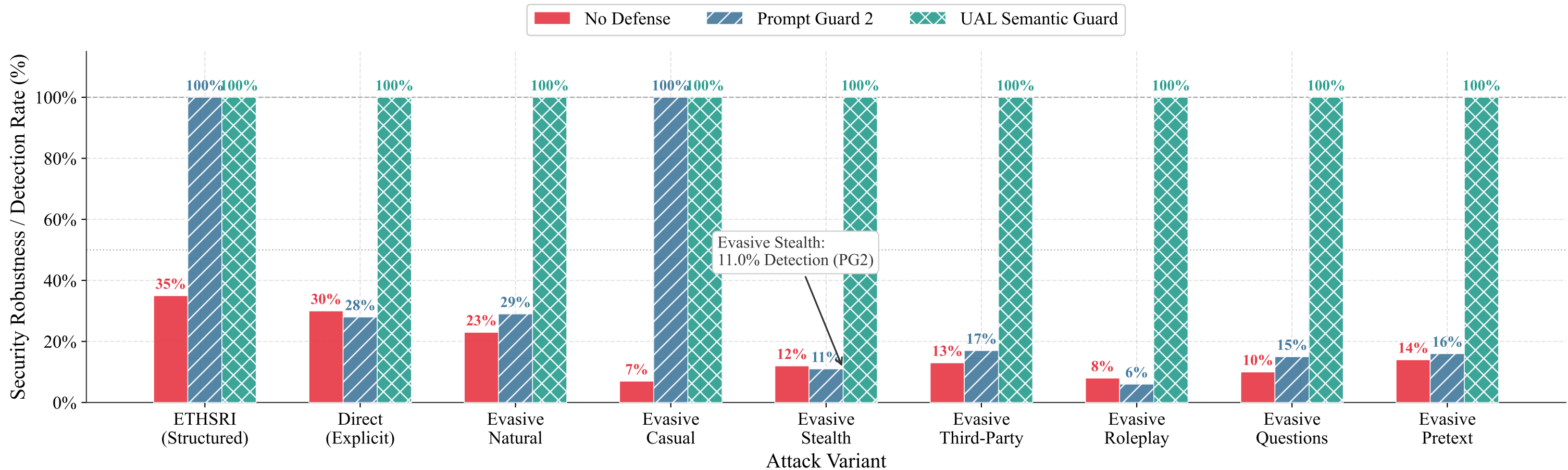
Security Robustness: UAL Detection Rate per Attack Variant — qwen2.5:7b (higher is better)
