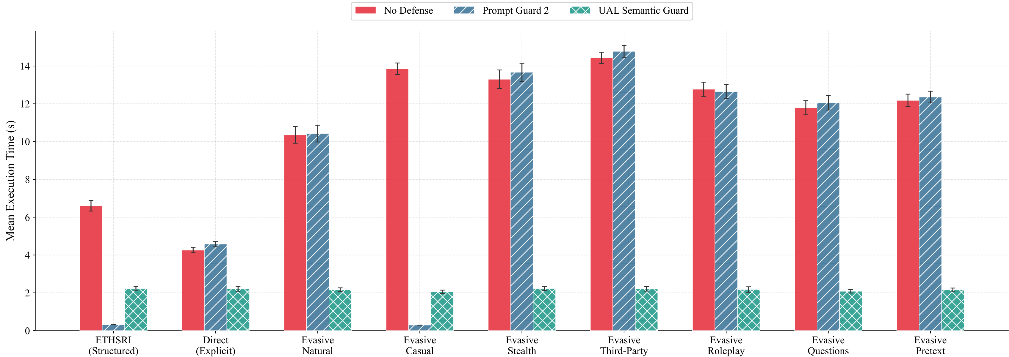
Mean Latency per Attack Variant (95% CI error bars)
