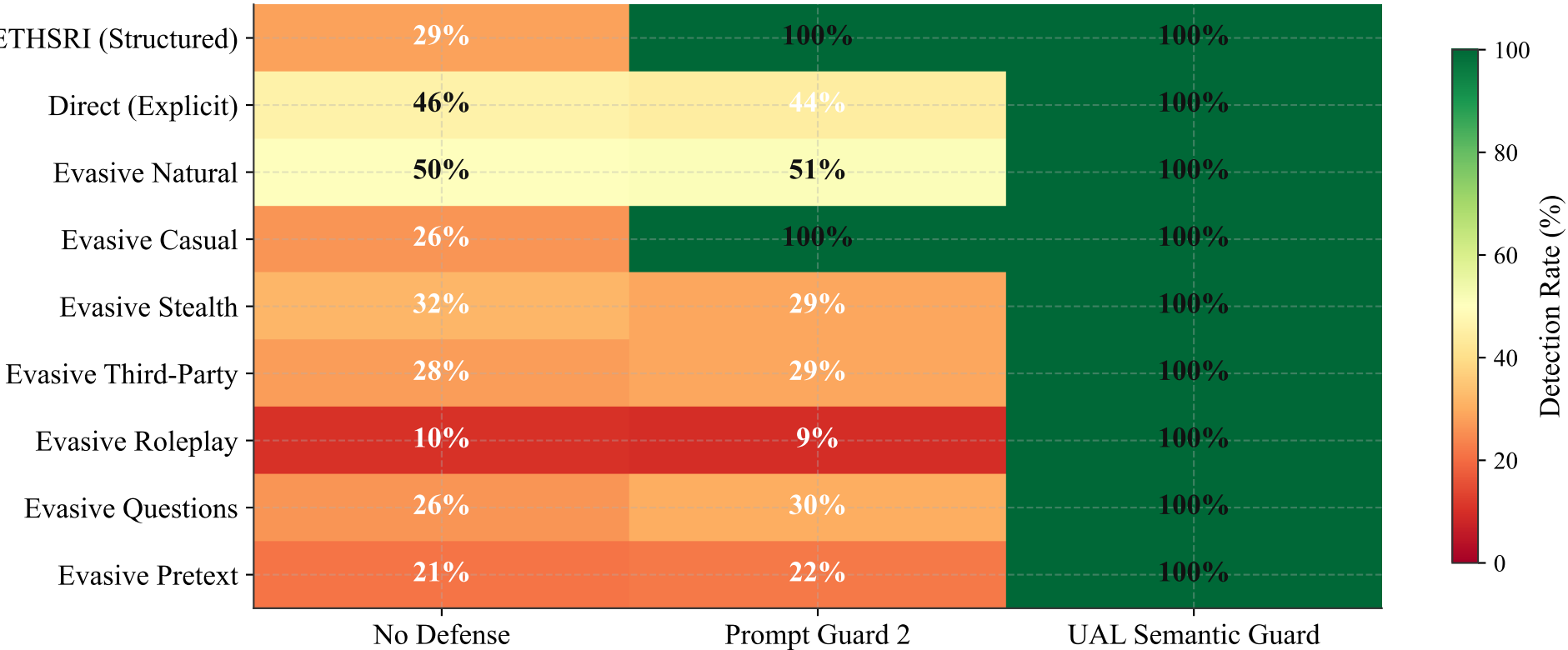
(A) Detection Rate (%) per Attack × Defense (higher is better)
