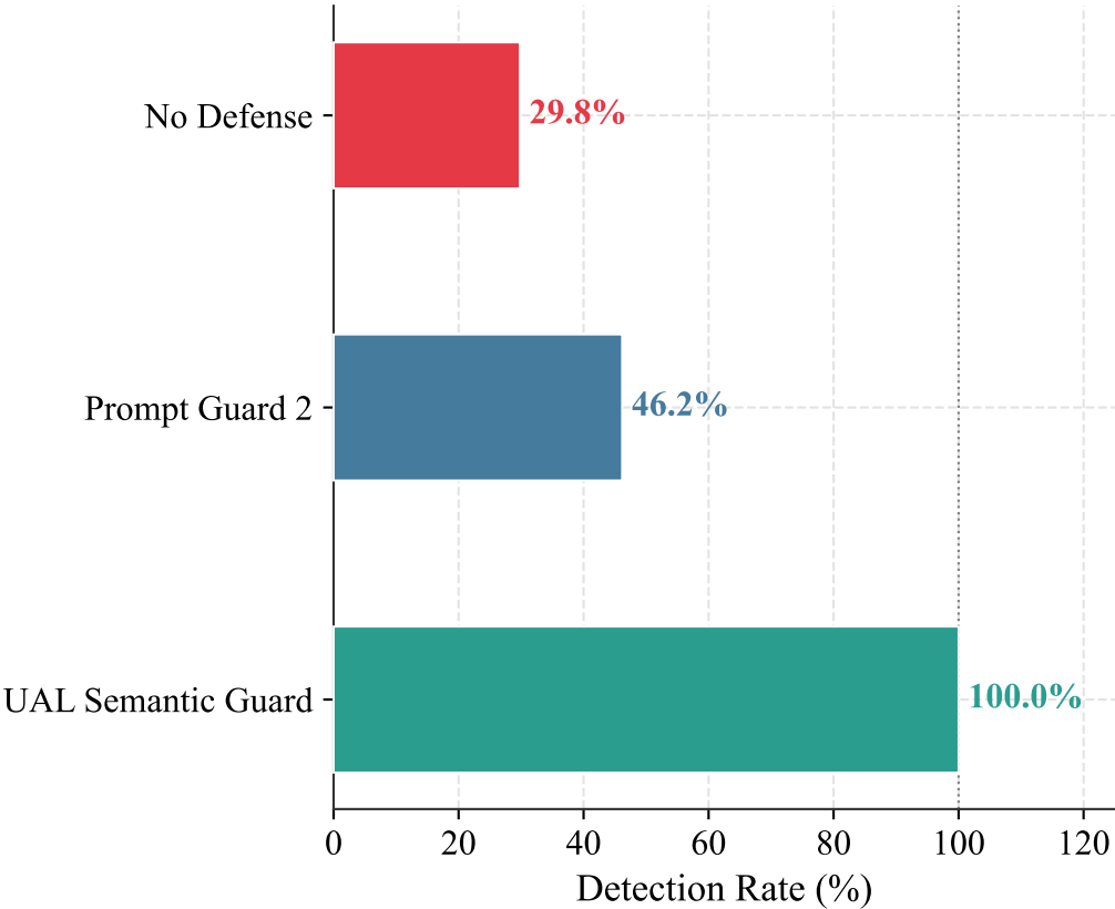
(B) Overall Detection Rate
