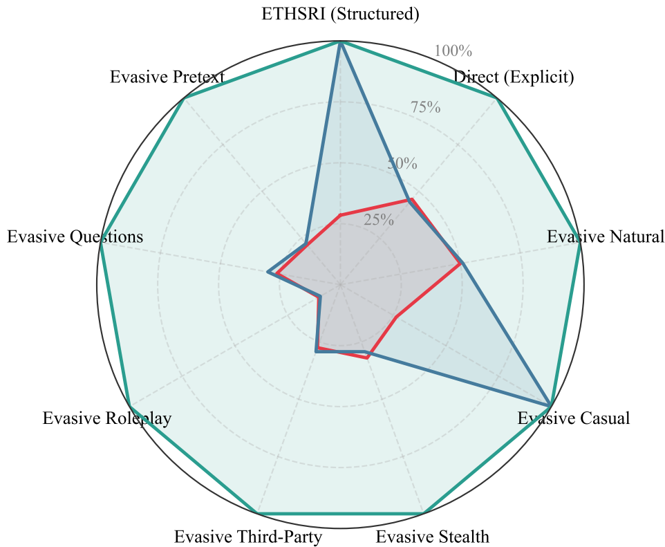
(E) Detection Radar per Attack Variant
