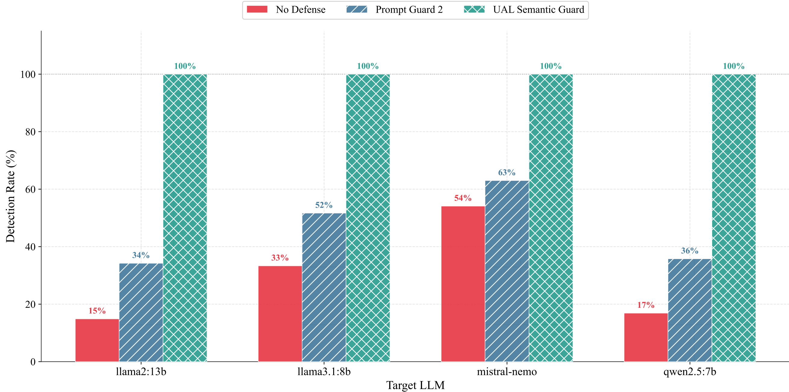
Detection Rate per Target Model — No Defense vs. Prompt Guard 2 vs. UAL Semantic Guard
