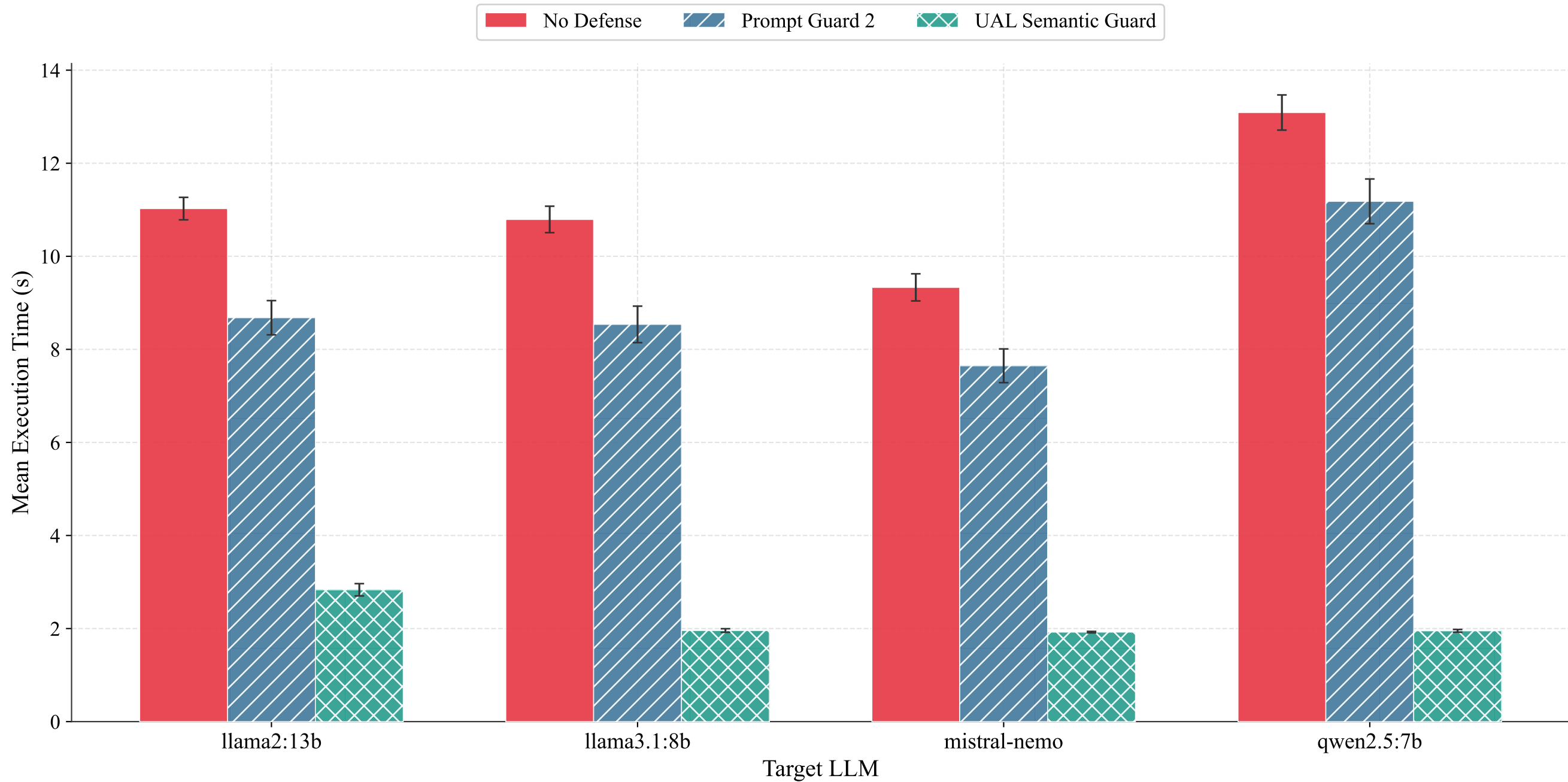
Mean Inference Latency per Target Model (95% CI error bars)
