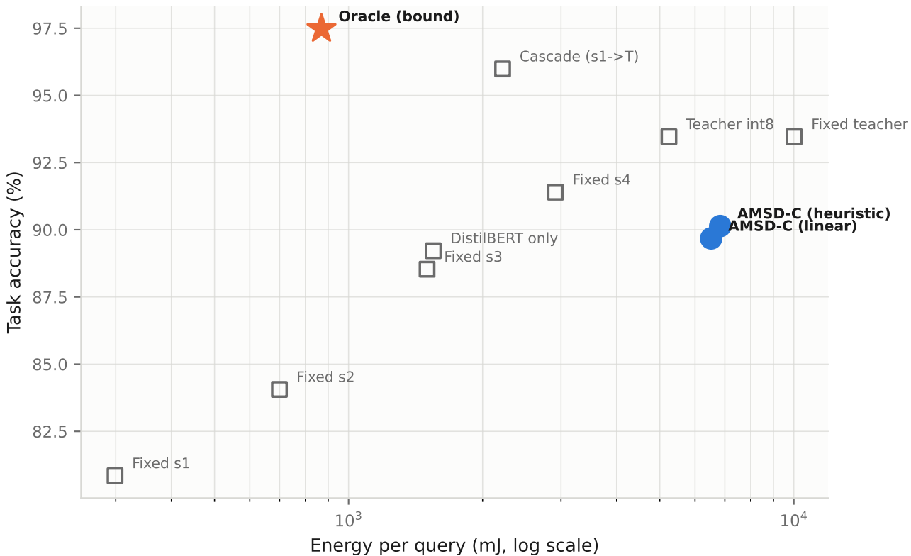
Energy-accuracy trade-off, SST2 · lower-left is cheaper, upper is better
