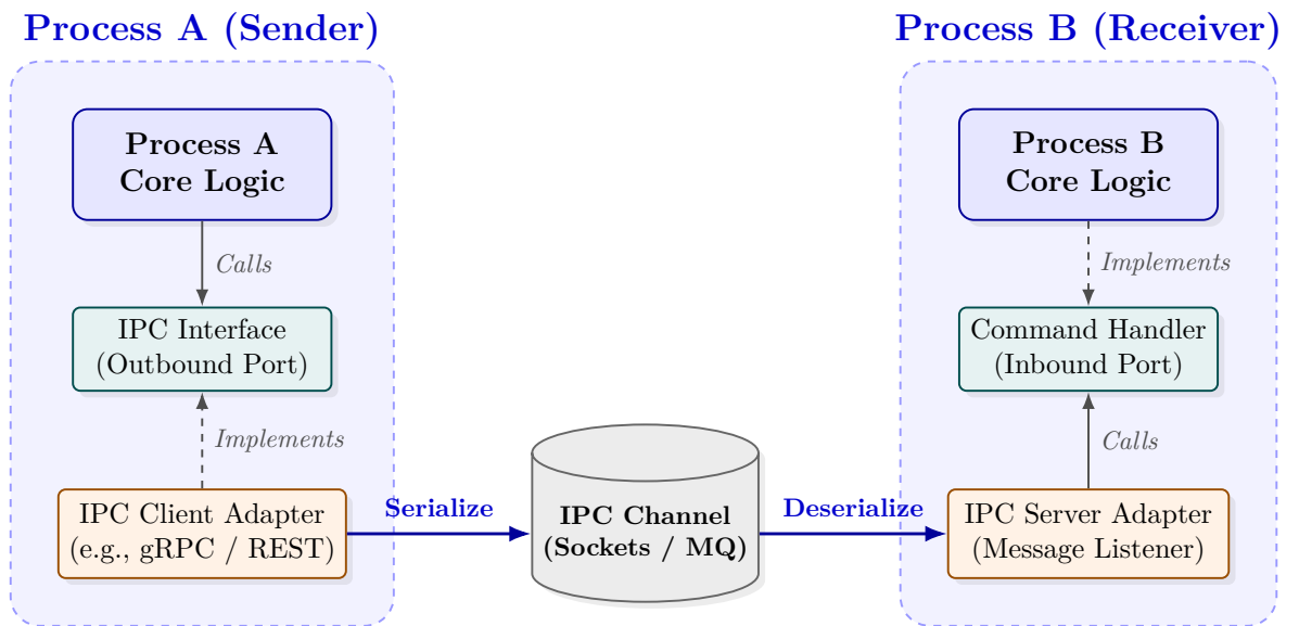
Figure 1: Inter-Process Communication flow. Core business logic is strictly isolated from network and serialization layers via Interface Ports.
