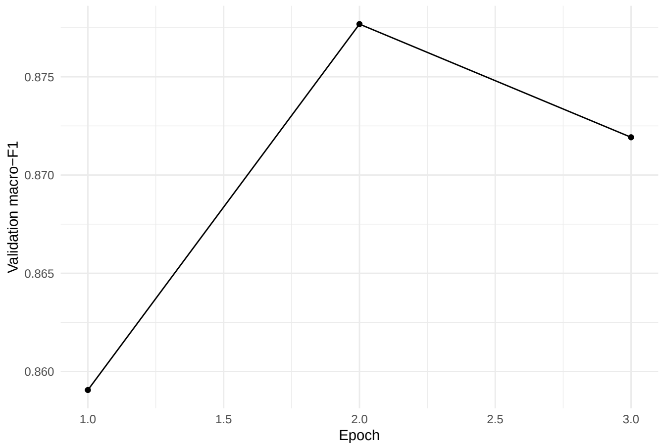
Fine-tuned BERT: validation macro-F1 by epoch
