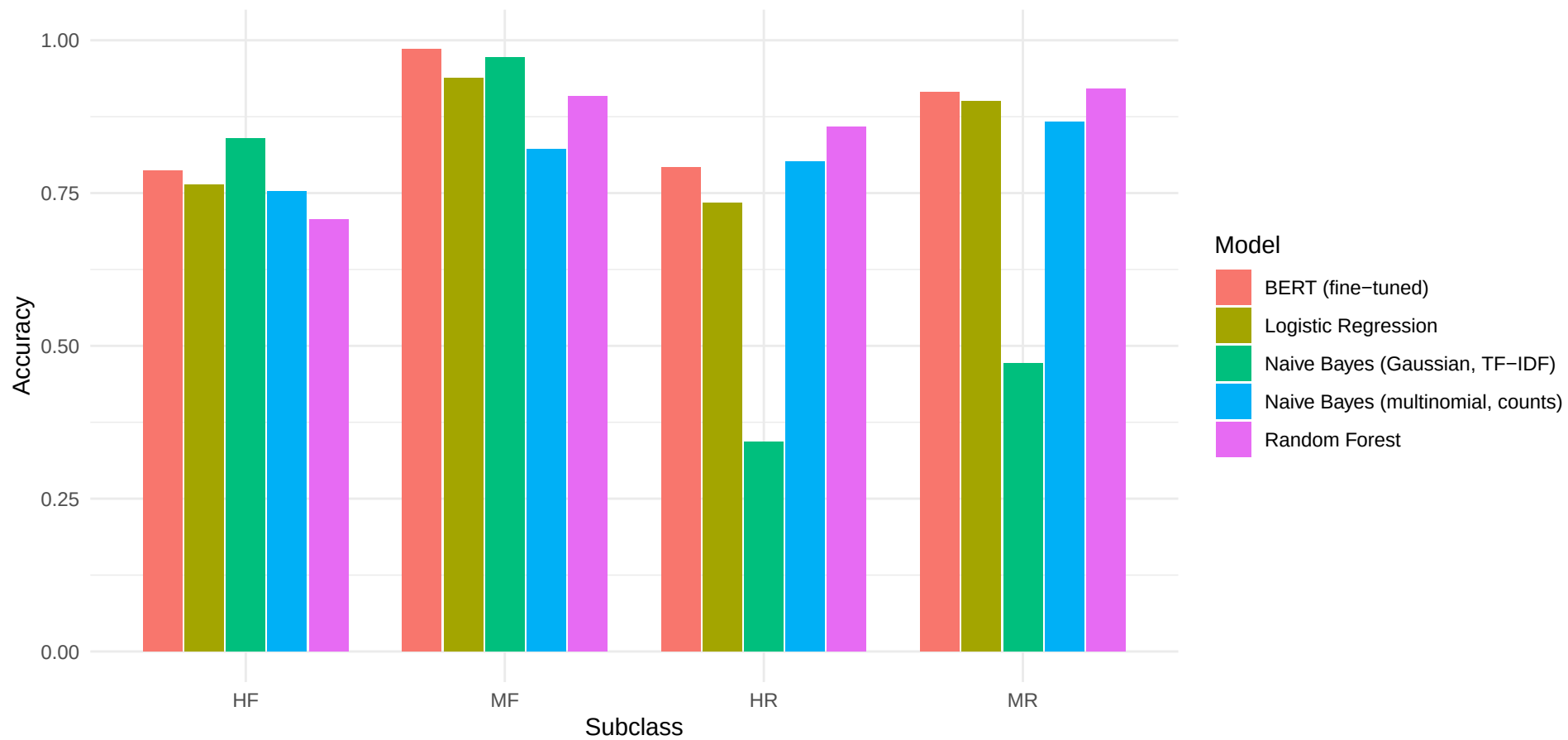
Subclass accuracy by detector
