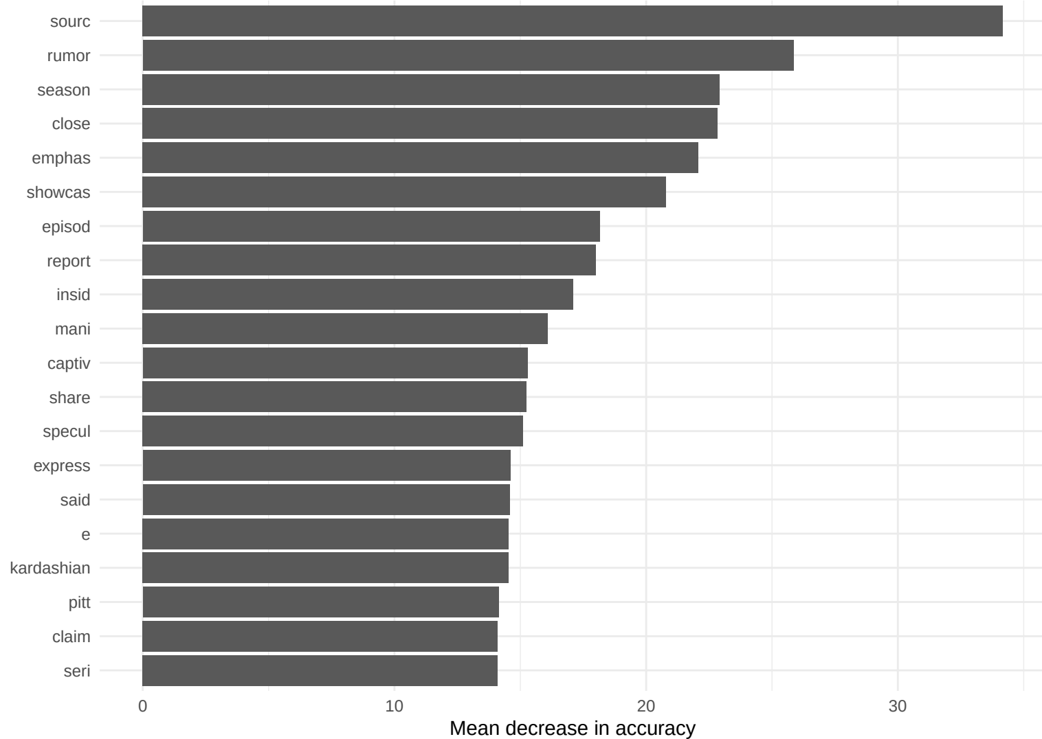
Random Forest: Top-20 features (permutation importance)
