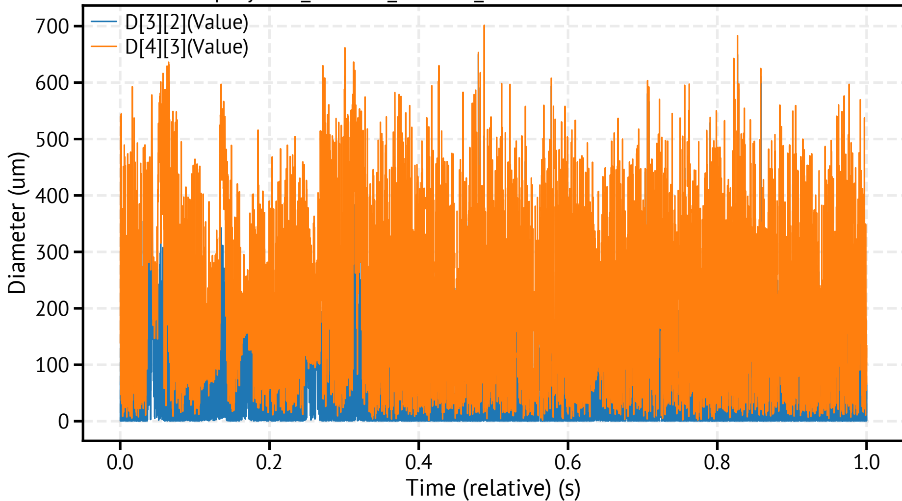
spraytec2_260310_142635_505800.csv - Mean Diameters
