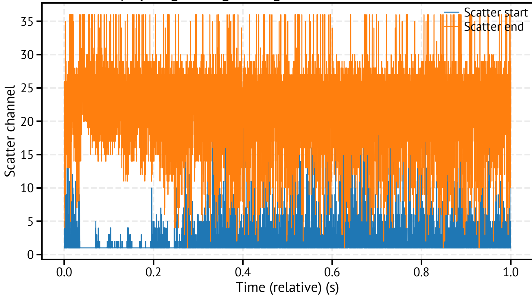
spraytec5_260310_142759_099200.csv - Scatter Start/End
