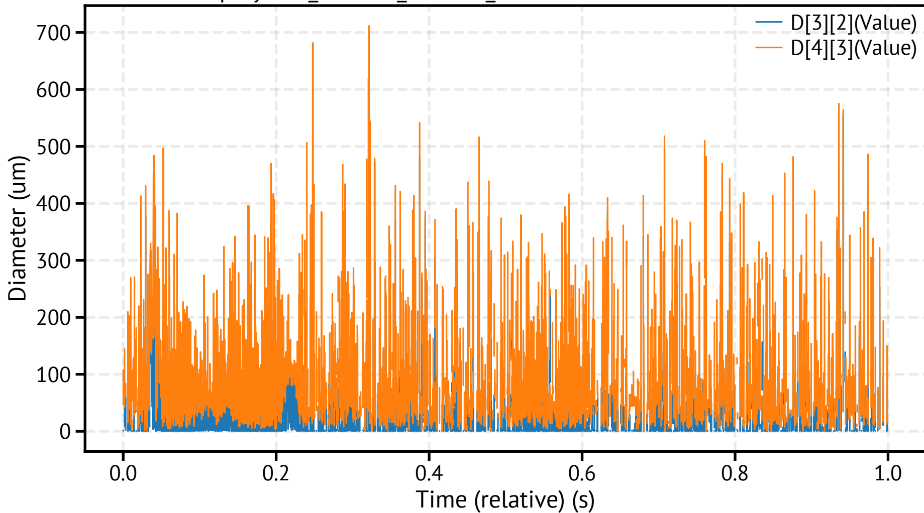
spraytec2_260310_164143_179600.csv - Mean Diameters
