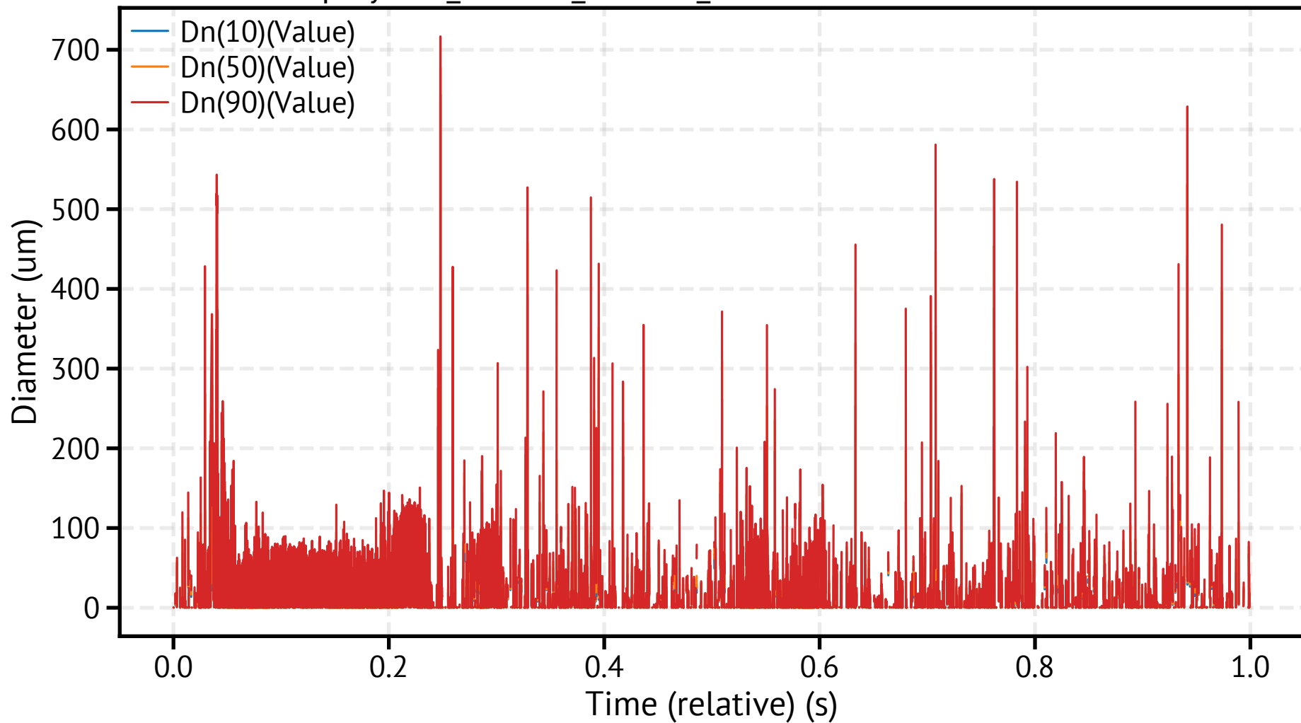
spraytec2_260310_164143_179600.csv - Dn Percentiles
