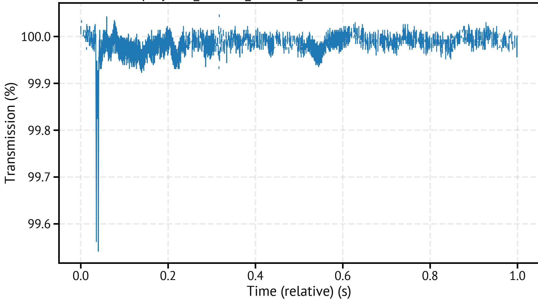
spraytec2_260310_164143_179600.csv - Transmission
