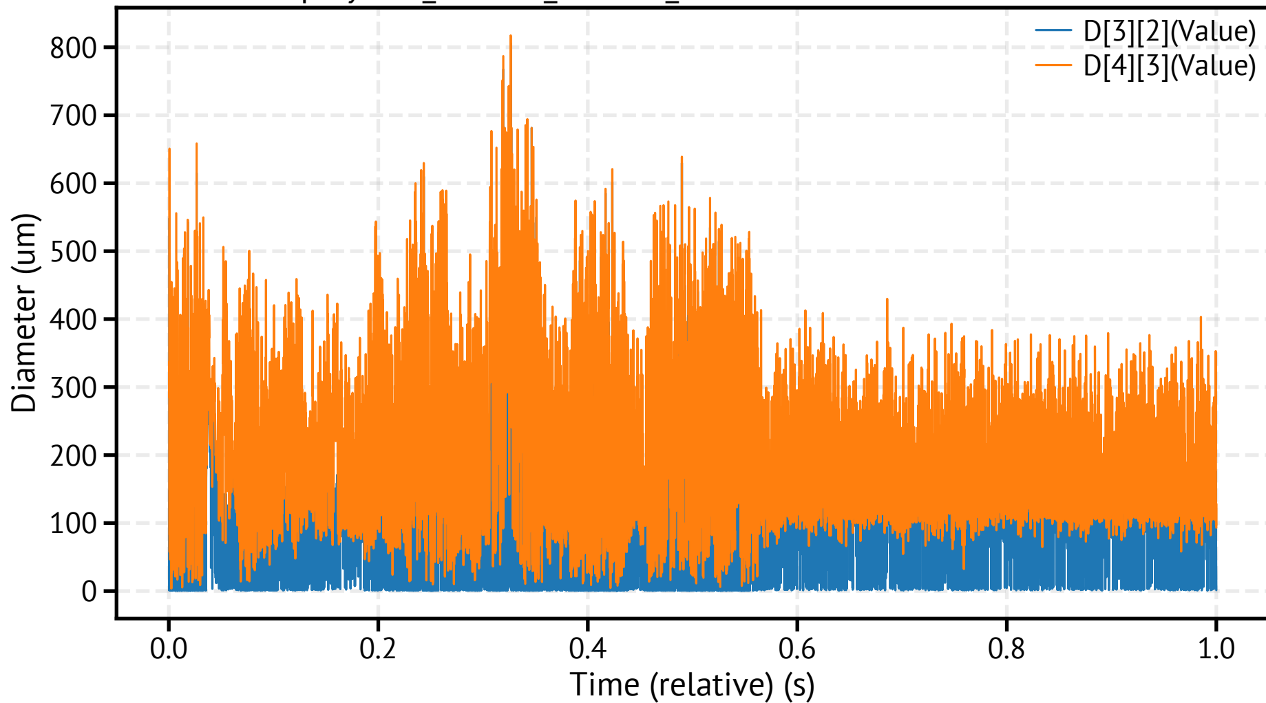
spraytec1_260310_165959_700100.csv - Mean Diameters
