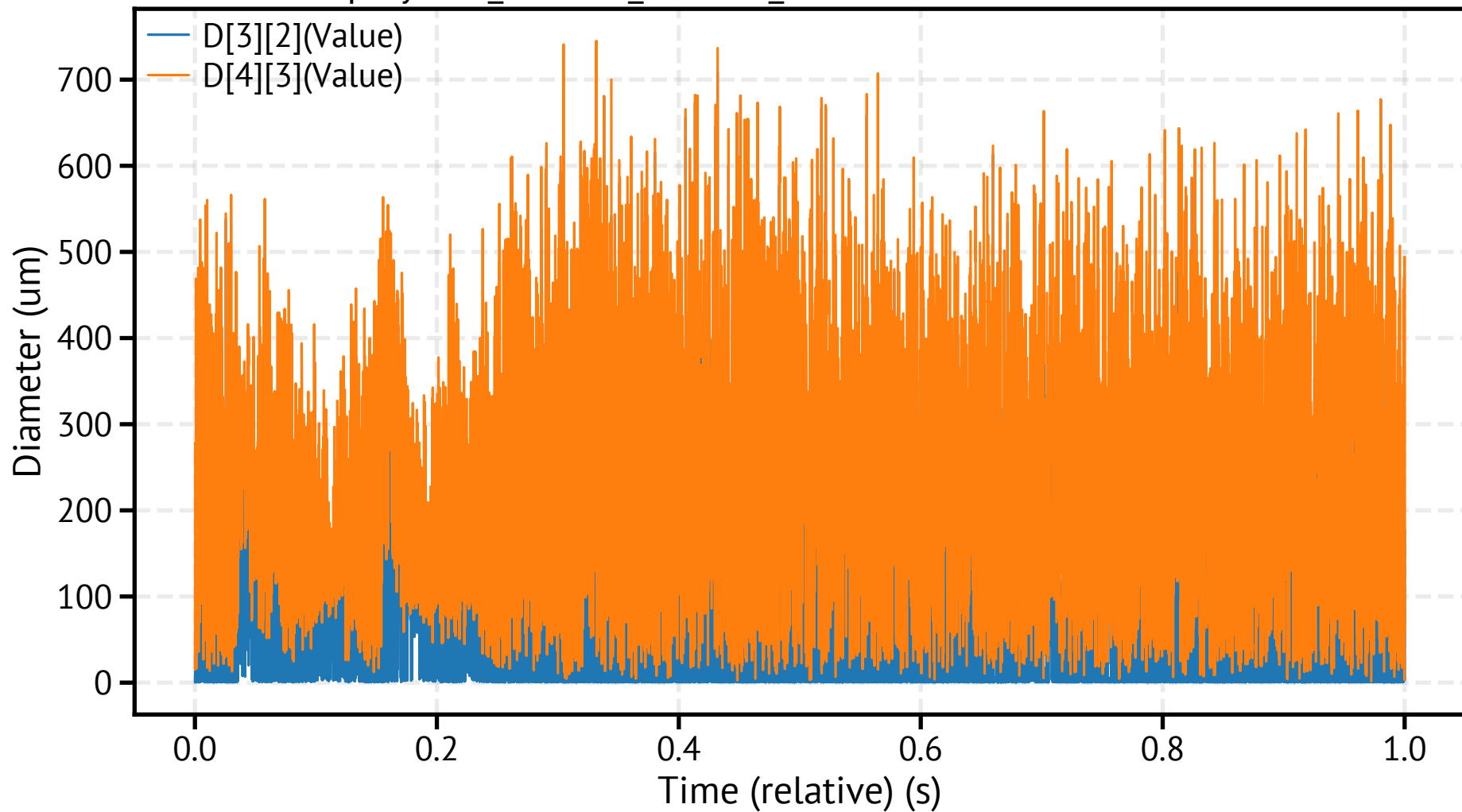
spraytec2_260310_170027_542400.csv - Mean Diameters
