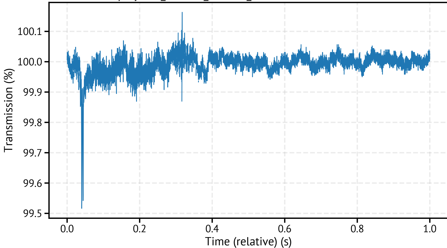
spraytec2_260310_170027_542400.csv - Transmission
