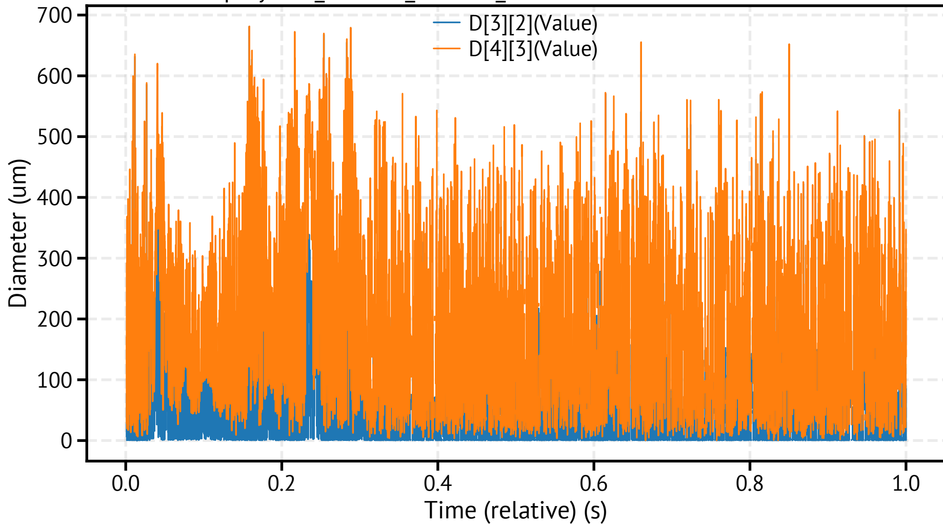
spraytec5_260311_151429_945300.csv - Mean Diameters
