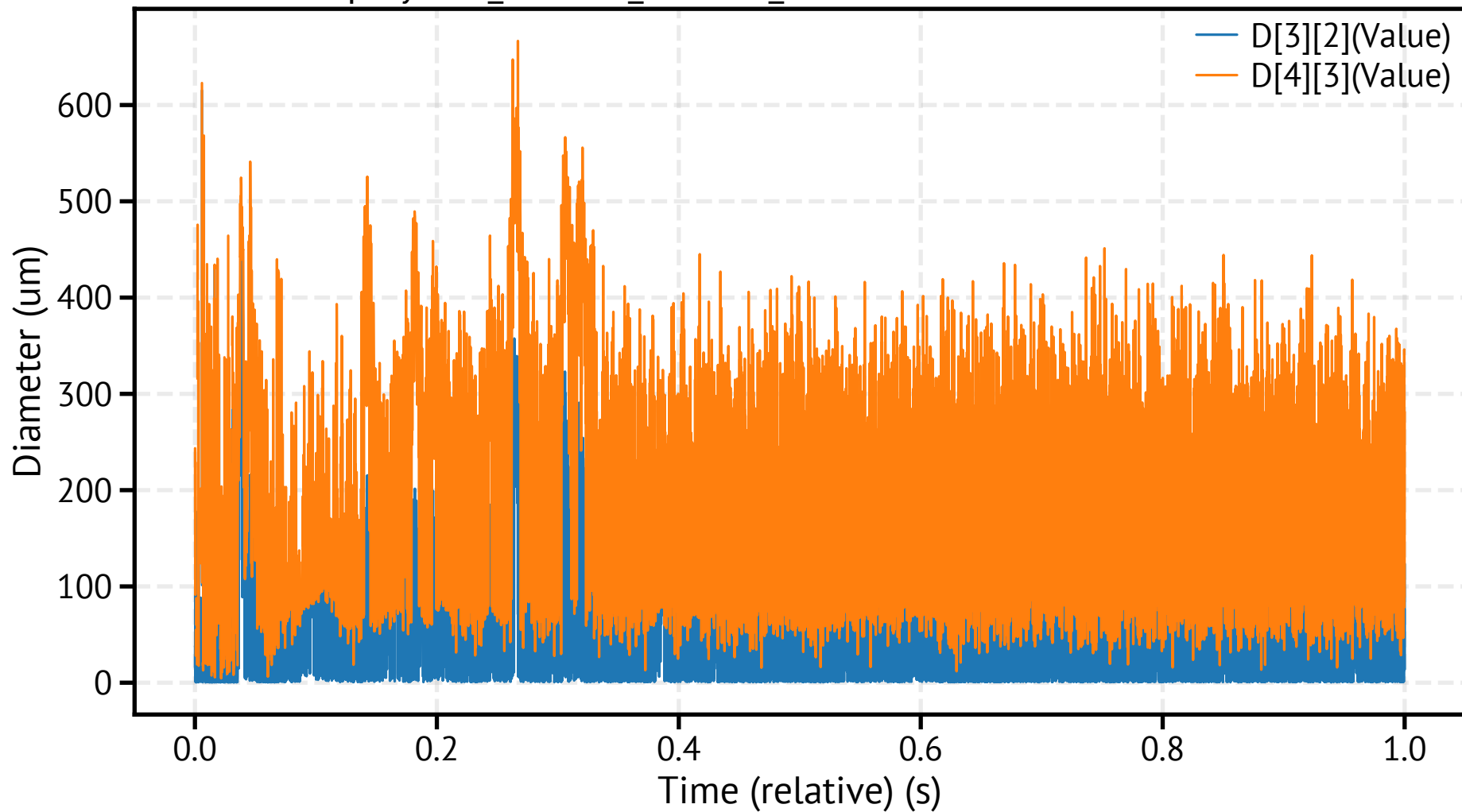
spraytec6_260311_151457_925300.csv - Mean Diameters
