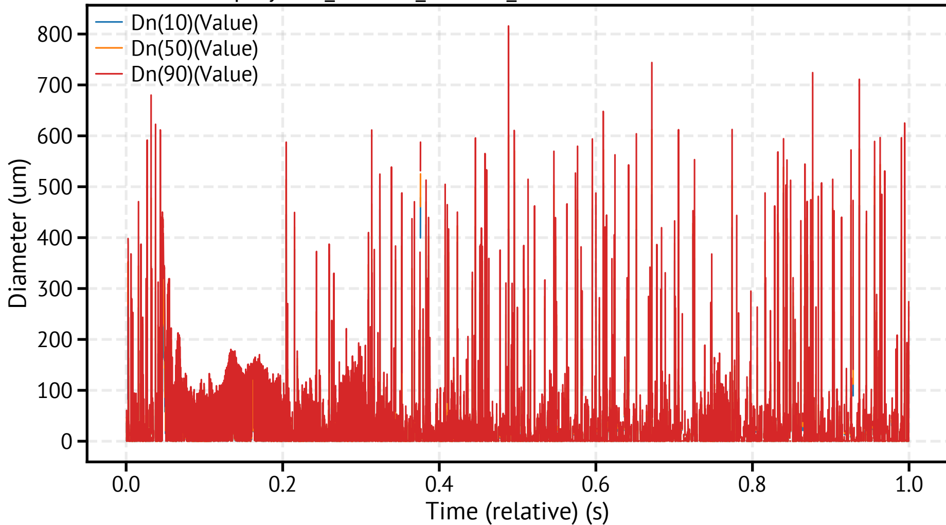
spraytec1_260318_095228_714300.csv - Dn Percentiles
