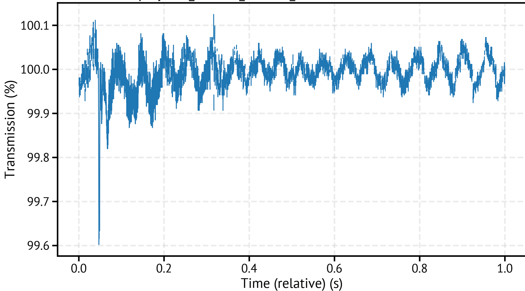
spraytec1_260318_095228_714300.csv - Transmission
