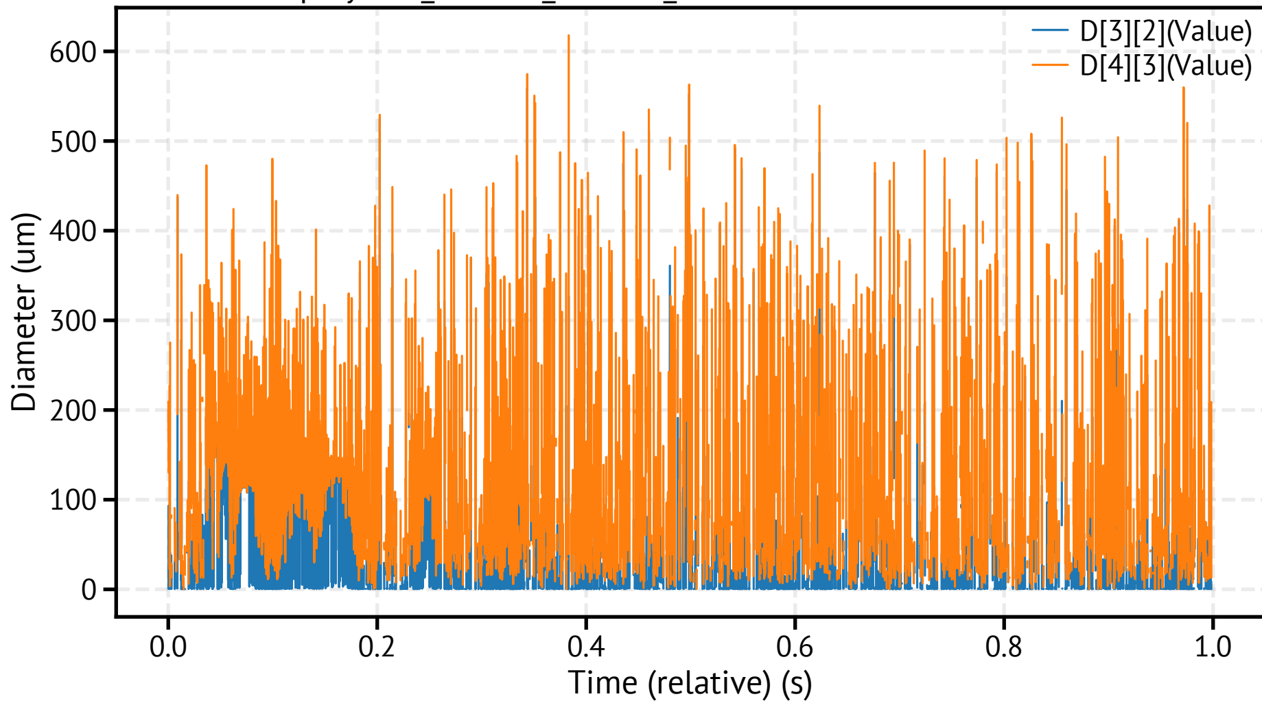
spraytec2_260318_095326_171900.csv - Mean Diameters
