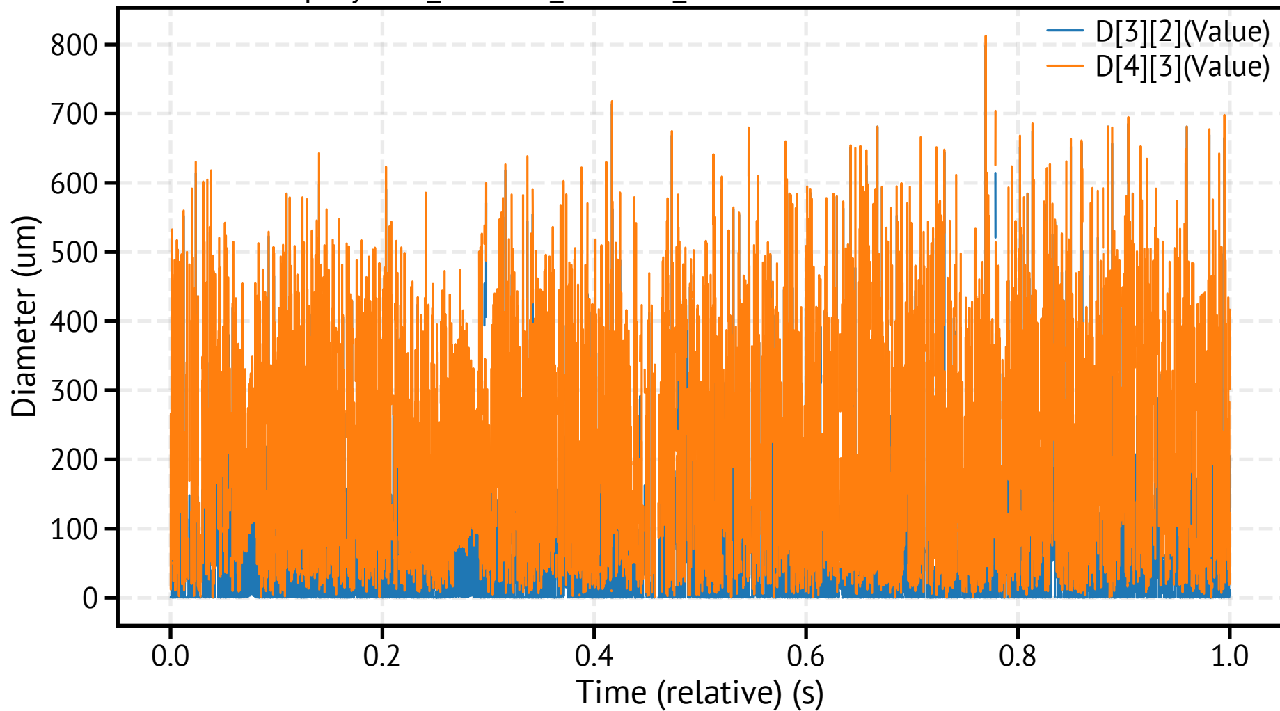
spraytec4_260318_095521_208200.csv - Mean Diameters
