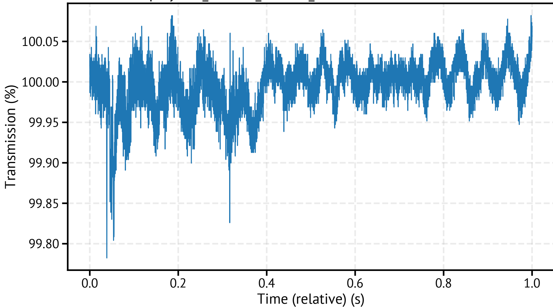
spraytec5_260318_095618_798700.csv - Transmission
