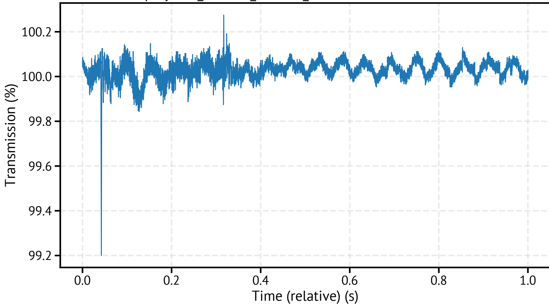
spraytec7_260318_095813_867700.csv - Transmission
